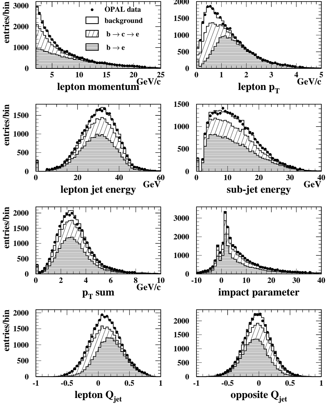
Figure 1: The eight input variables used by the neural networks NN_{b\ell} and NN_{bc\ell} to separate b \rightarrow \ell and b \rightarrow c \rightarrow \ell decays. The contributions from the three classes of Monte Carlo events; b \rightarrow \ell , b \rightarrow c \rightarrow \ell and backgrounds, are superimposed and compared to the data after normalisation and rescaling using the fractions f(b \rightarrow \ell) and f(b \rightarrow c \rightarrow \ell) derived in Section 5.2. The results are shown here for electrons only.
