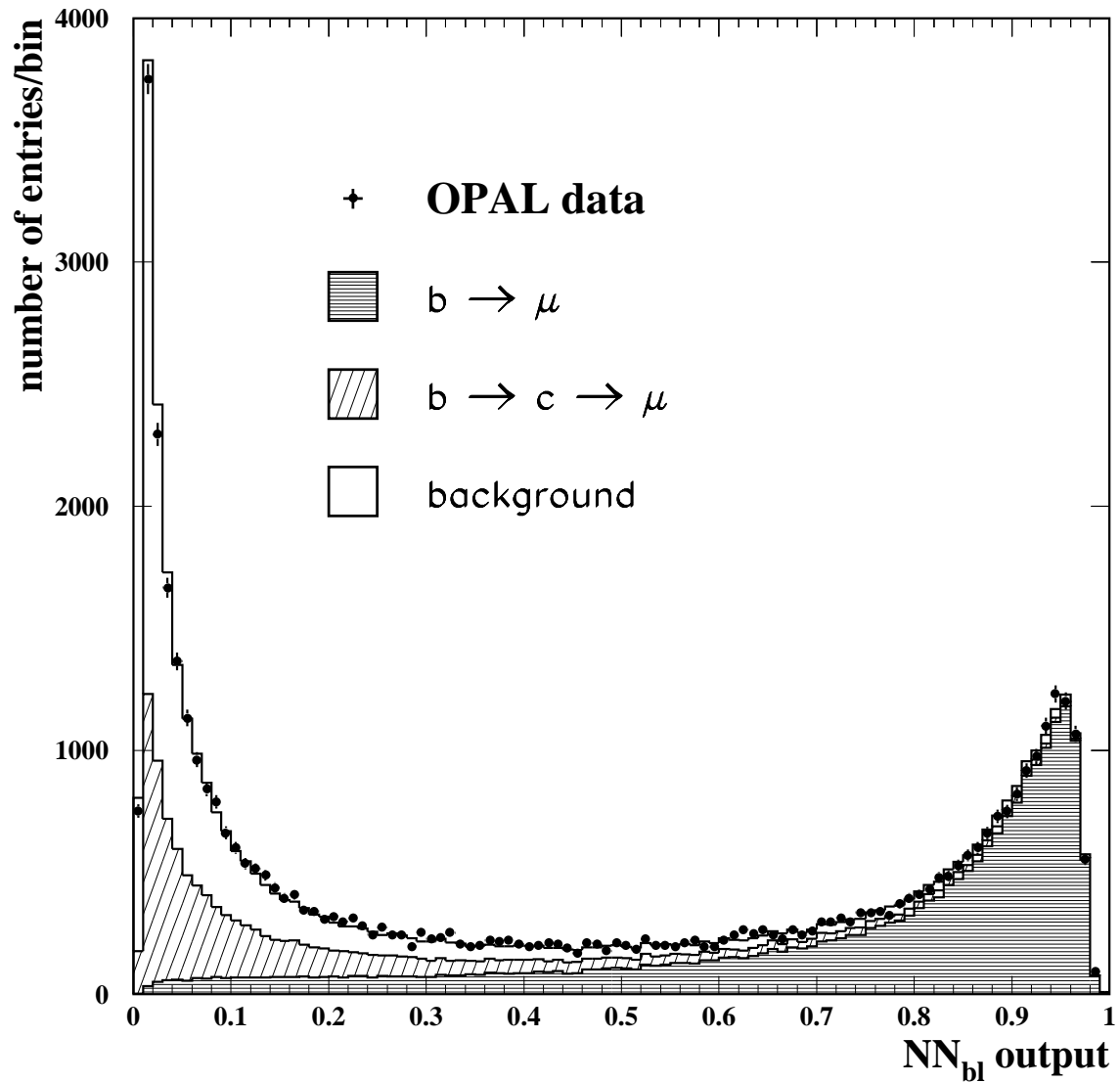
Figure 2: Distribution of the output variable for the neural network NN_{b\ell} trained specifically to distinguish b \rightarrow \ell events from all other types of events. The three categories b \rightarrow \ell , b \rightarrow c \rightarrow \ell , and background are described in the text. The results are shown here for muons only.
