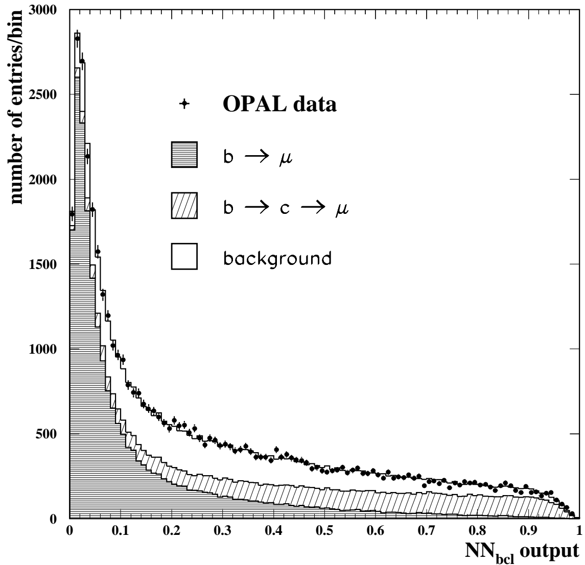
Figure 3: Distribution of the output variable for the neural network \text{NN}_{bcl} trained specifically to distinguish b \rightarrow c \rightarrow \ell events from all other types of events. The three categories b \rightarrow \ell , b \rightarrow c \rightarrow \ell , and background are described in the text. The results are shown here for muons only.
