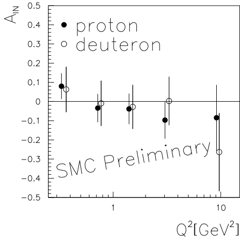
Figure 4. A_{LL}^{lN \rightarrow \rho^0 l' N} for p_T^2 > 0.09 \text{ GeV}^2/c^2 (the errors are statistical only).
