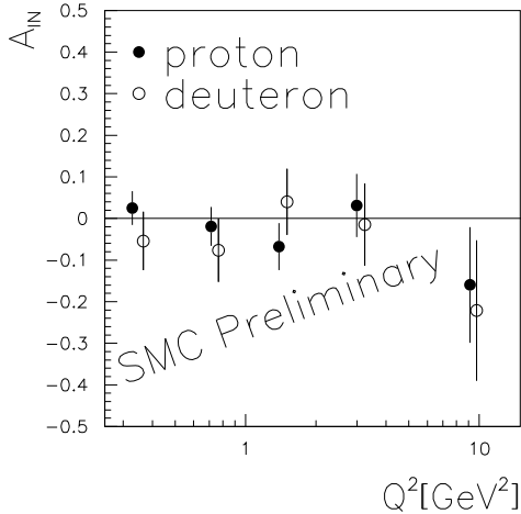
Figure 3. A_{LL}^{lN \rightarrow \rho^0 l' N} for proton and deuteron as a function of Q^2 (the errors are statistical only).
