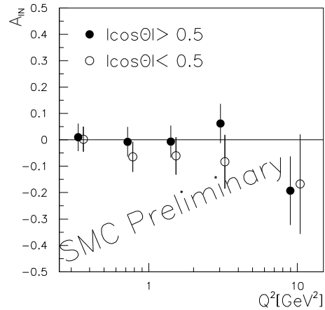
Figure 5. A_{LL}^{lN \rightarrow \rho^0 l' N} for |\cos \vartheta| > 0.5 and |\cos \vartheta| < 0.5 for proton and deuteron combined (the errors are statistical only).
