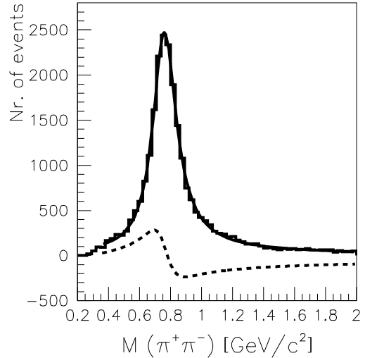
Figure 2. Mass spectrum (1995 data) after selections. The full line represents a fit according to the Söding model, the dotted line the interference term between the resonant and non resonant amplitudes.
