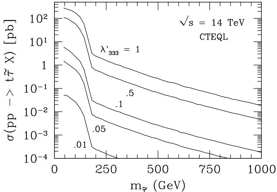
FIG. 10. The leading-order production cross section \sigma(pp \rightarrow t\tilde{\tau}X) , for \sqrt{s} = 14\text{TeV} , as a function of the \tilde{\tau} mass is shown for different values of \lambda'_{333} . Renormalization and factorization scales are fixed as \mu_R = \mu_f = m_t + m_{\tilde{\tau}} .
