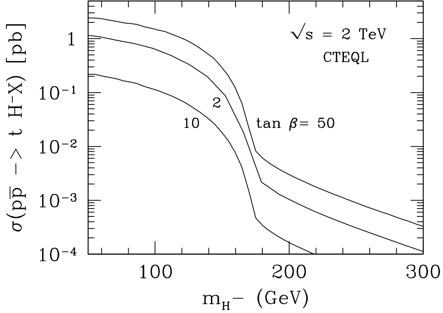
FIG. 7. The leading-order production cross section \sigma(p\bar{p} \rightarrow tH^-X) , for \sqrt{s} = 2\text{TeV} , as a function of the charged Higgs mass, is shown for three different values of \tan\beta = 2, 10, 50 . The cross section is obtained by adding the contribution of the 2 \rightarrow 2 process, gb \rightarrow tH^- , to those of the 2 \rightarrow 3 ones, gg \rightarrow t\bar{b}H^- and q\bar{q} \rightarrow t\bar{b}H^- , and subtracting overlapping terms. Renormalization and factorization scales are fixed as \mu_R = \mu_f = m_t + m_{H^-} .
