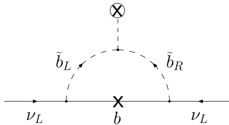
FIG. 11. A one-loop contribution to the Majorana neutrino mass arising from the \Delta L = 1 operators of the superpotential (9).
