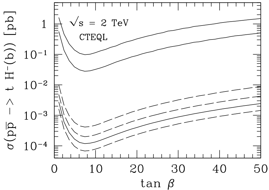
FIG. 4. The production cross section \sigma(p\bar{p} \rightarrow t(\bar{b})H^-X) is shown as a function of \tan\beta for m_{H^\pm} = 100, 140, \text{ and } 200\text{ GeV} (from top to bottom). As in Fig. 3, solid lines correspond to the 2 \rightarrow 3 processes, dashed lines to the 2 \rightarrow 2 process.
