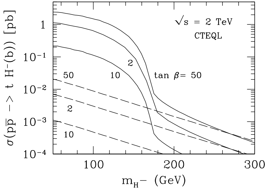
FIG. 3. The leading-order production cross section \sigma(p\bar{p} \rightarrow t(\bar{b})H^-X) as a function of the charged Higgs mass, for \sqrt{s} = 2\text{ TeV} , is shown for three different values of \tan\beta = 2, 10, 50 . The solid lines indicate the cross sections obtained from 2 \rightarrow 3 elementary processes gg \rightarrow t\bar{b}H^- and q\bar{q} \rightarrow t\bar{b}H^- ; the dashed lines show the cross sections obtained from the 2 \rightarrow 2 process gb \rightarrow tH^- . Renormalization and factorization scales are fixed as \mu_R = \mu_f = m_t + m_{H^-} .
