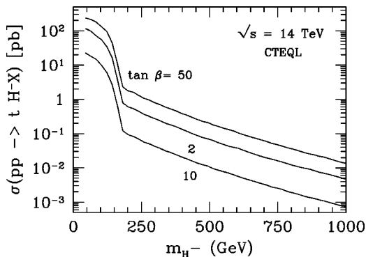
FIG. 8. Same as in Fig. 7 for center-of-mass energy \sqrt{s} = 14 TeV.
