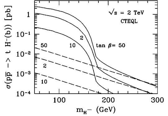
FIG. 3. The leading-order production cross section \sigma(p\bar{p} \rightarrow t(\bar{b})H^- X) as a function of the charged Higgs mass, for \sqrt{s} = 2 TeV, is shown for three different values of \tan \beta = 2, 10, 50 . The solid lines indicate the cross sections obtained from 2 \rightarrow 3 elementary processes gg \rightarrow t\bar{b}H^- and q\bar{q} \rightarrow t\bar{b}H^- ; the dashed lines show the cross sections obtained from the 2 \rightarrow 2 process gb \rightarrow tH^- . Renormalization and factorization scales are fixed as \mu_R = \mu_f = m_t + m_{H^-} .
