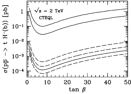
FIG. 4. The production cross section \sigma(pp \rightarrow t(\bar{b})H^- X) is shown as a function of \tan\beta for m_{H^\pm} = 100, 140, and 200 GeV (from top to bottom). As in Fig. 3, solid lines correspond to the 2 \rightarrow 3 processes; dashed lines to the 2 \rightarrow 2 process.
