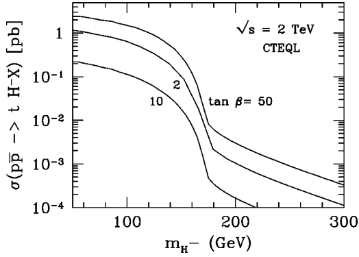
FIG. 7. The leading-order production cross section \sigma(p\bar{p} \rightarrow tH^-X) , for \sqrt{s}=2 TeV, as a function of the charged Higgs mass, is shown for three different values of \tan\beta=2,10,50 . The cross section is obtained by adding the contribution of the 2→2 process, gb \rightarrow tH^- , to those of the 2→3 ones, gg \rightarrow t\bar{b}H^- and q\bar{q} \rightarrow t\bar{b}H^- , and subtracting overlapping terms. Renormalization and factorization scales are fixed as \mu_R = \mu_f = m_t + m_{H^-} .
