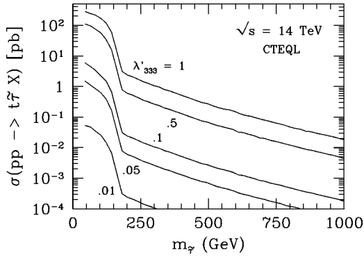
FIG. 10. The leading-order production cross section \sigma(pp \rightarrow t\tilde{\tau}X) , for \sqrt{s}=14 TeV, as a function of the \tilde{\tau} mass is shown for different values of \lambda'_{333} . Renormalization and factorization scales are fixed as \mu_R = \mu_f = m_t + m_{\tilde{\tau}} .
