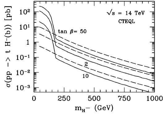
FIG. 5. The leading-order production cross section \sigma(pp \rightarrow t(\bar{b})H^- X) , for \sqrt{s} = 14 TeV; is shown as a function of the charged Higgs mass for three different values of \tan\beta = 2, 10, 50 . As in Figs. 3 and 4, the solid lines indicate the cross sections obtained from 2 \rightarrow 3 elementary processes; the dashed lines, the cross sections obtained from the 2 \rightarrow 2 process. Renormalization and factorization scales are fixed as \mu_R = \mu_f = m_t + m_{H^-} .
