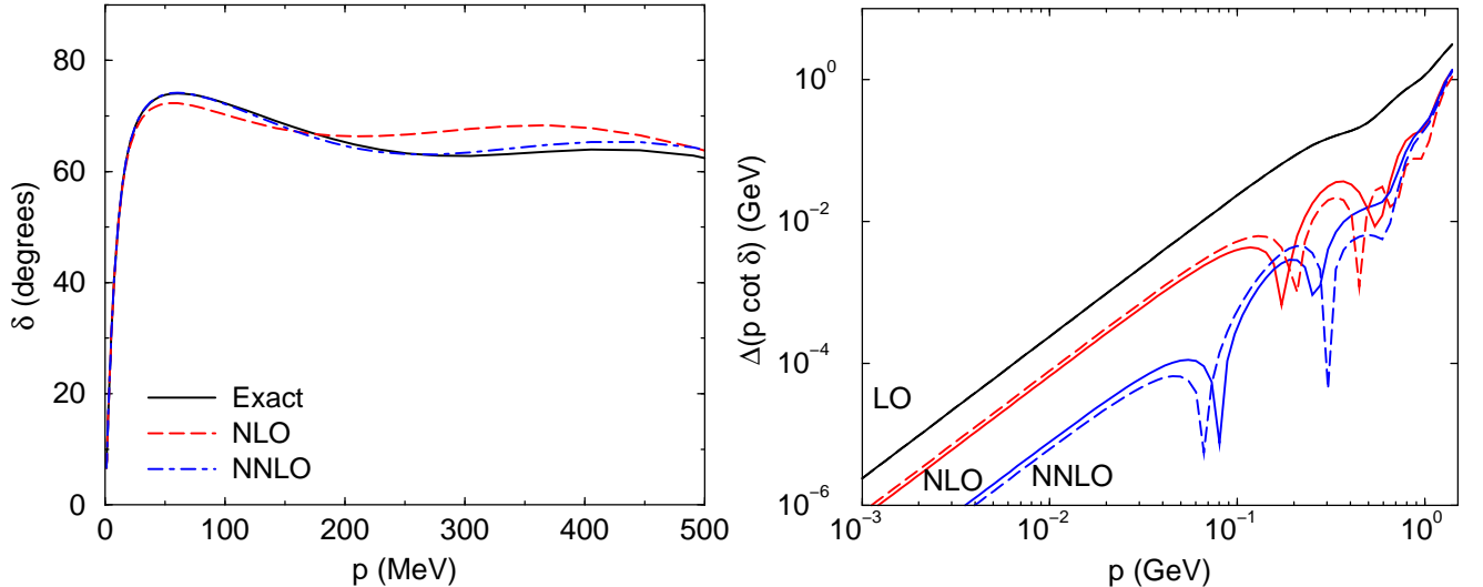
FIG. 2. The algorithm of §III C 3 for the KSW expansion applied to the two delta-shell model. The left plot shows that as more orders are added to the EFT calculation, the agreement with the exact phase shift improves. The right plot shows the corresponding errors in the observable p \cot \delta .
