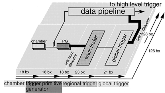
Fig. 3. Muon trigger track finder processor data chain. Numbers give the latency of the components.
