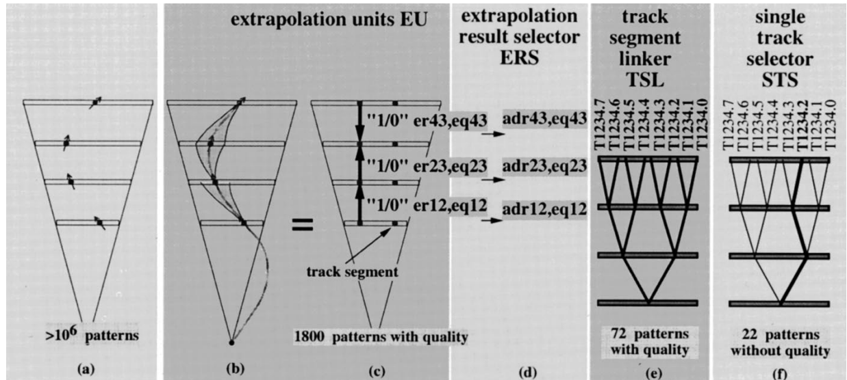
Fig. 16. Reduction of possible track candidates by the track finder algorithm.
