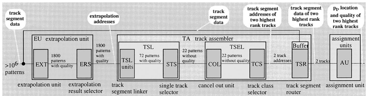
Fig. 15. Block diagram of a sector processor.
