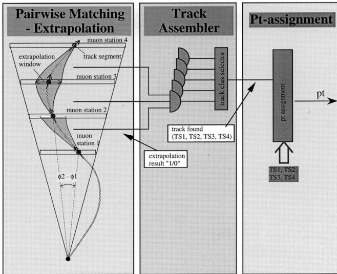
Fig. 5. Principle of the track finder algorithm (three-step scheme).
