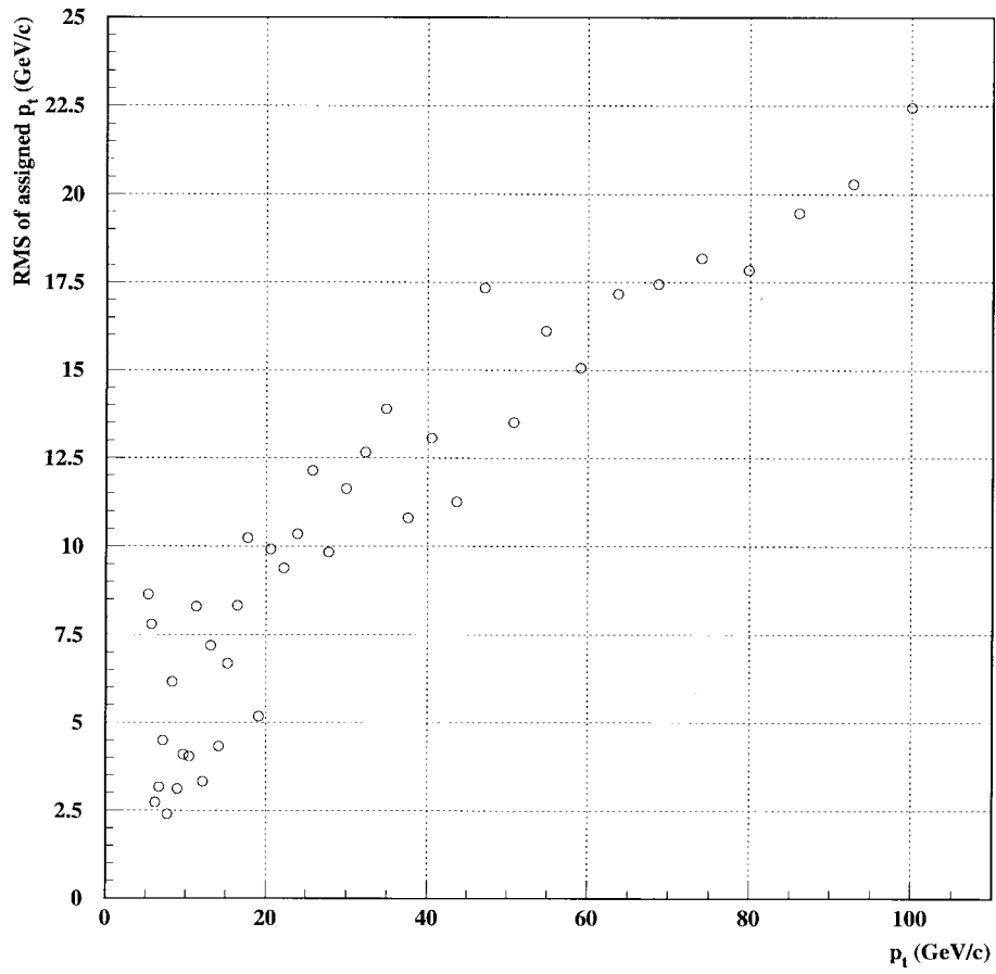
Fig. 12. Resolution of the transverse momentum p_t as a function of this momentum itself.
