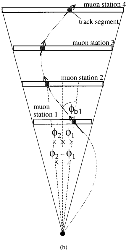
Fig. 9. (a) Matching track segment pairs are combined to a full track. (b) Using the deflection \phi_2 - \phi_1 or the bending angle \phi_b to determine p_t .
