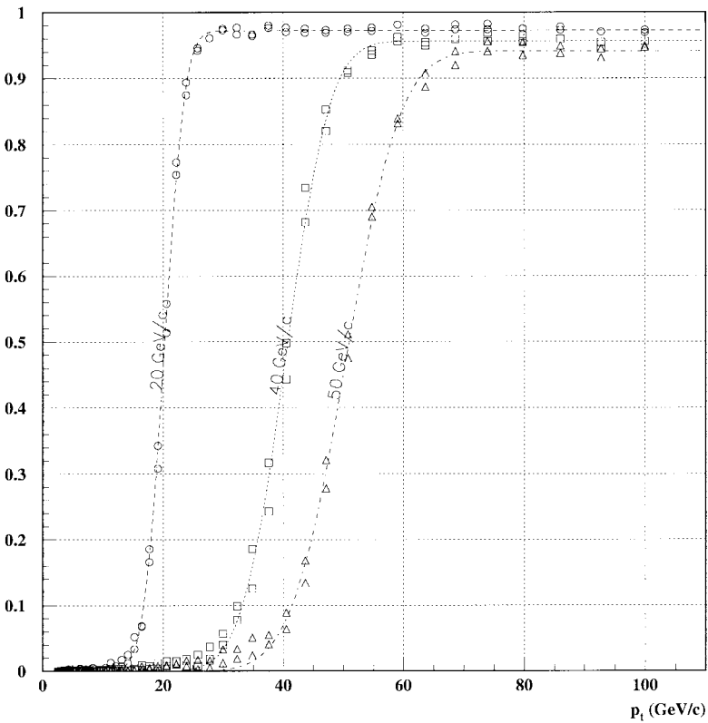
Fig. 13. Efficiency curves for p_t -thresholds of 20, 40, and 50 GeV/c. Higher thresholds are not likely to be needed.
