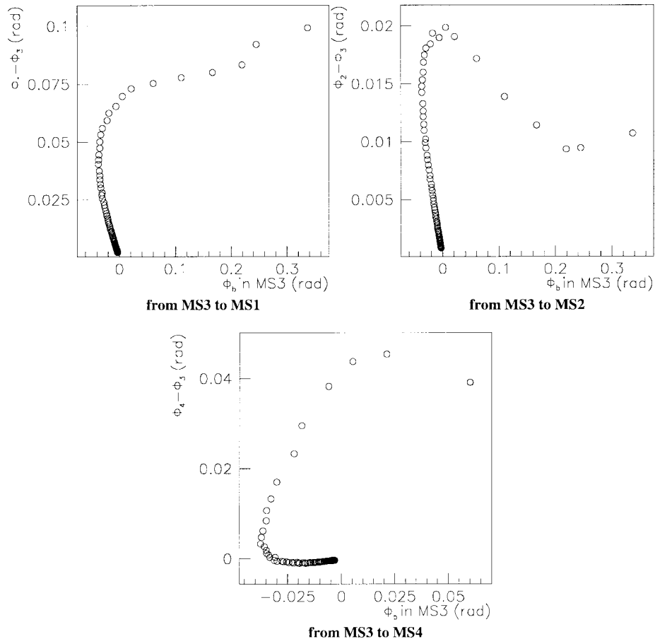
Fig. 8. Relationship between bend angle \phi_b in station three and deflection of the muon is ambiguous.
