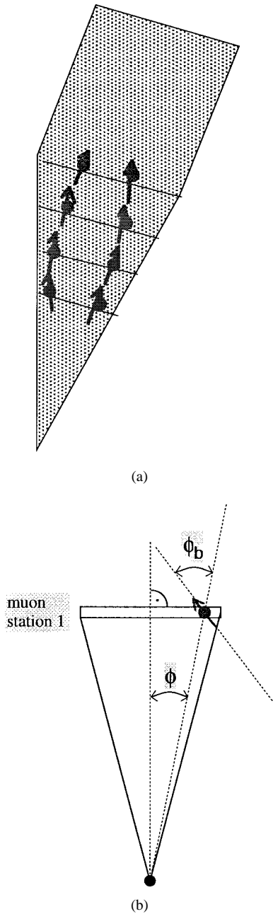
Fig. 2. (a) Up to two track segments per chamber are given out. (b) A track segment consists of the spatial coordinate f (11 bit), the bend angle \phi_b (8 bit), and quality (3 bit).
