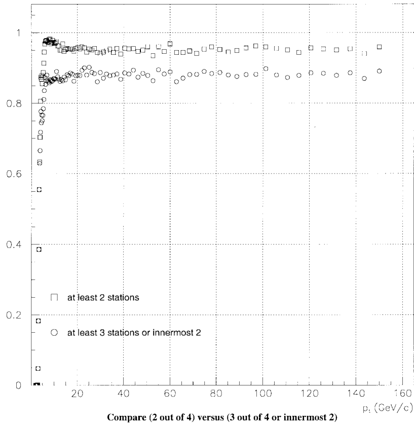
Fig. 10. This plot compares two track finder requirements. Circles show the case where a track has to have at least three track segments or track segments in the two innermost stations. Squares require only two track segments for a valid track.
