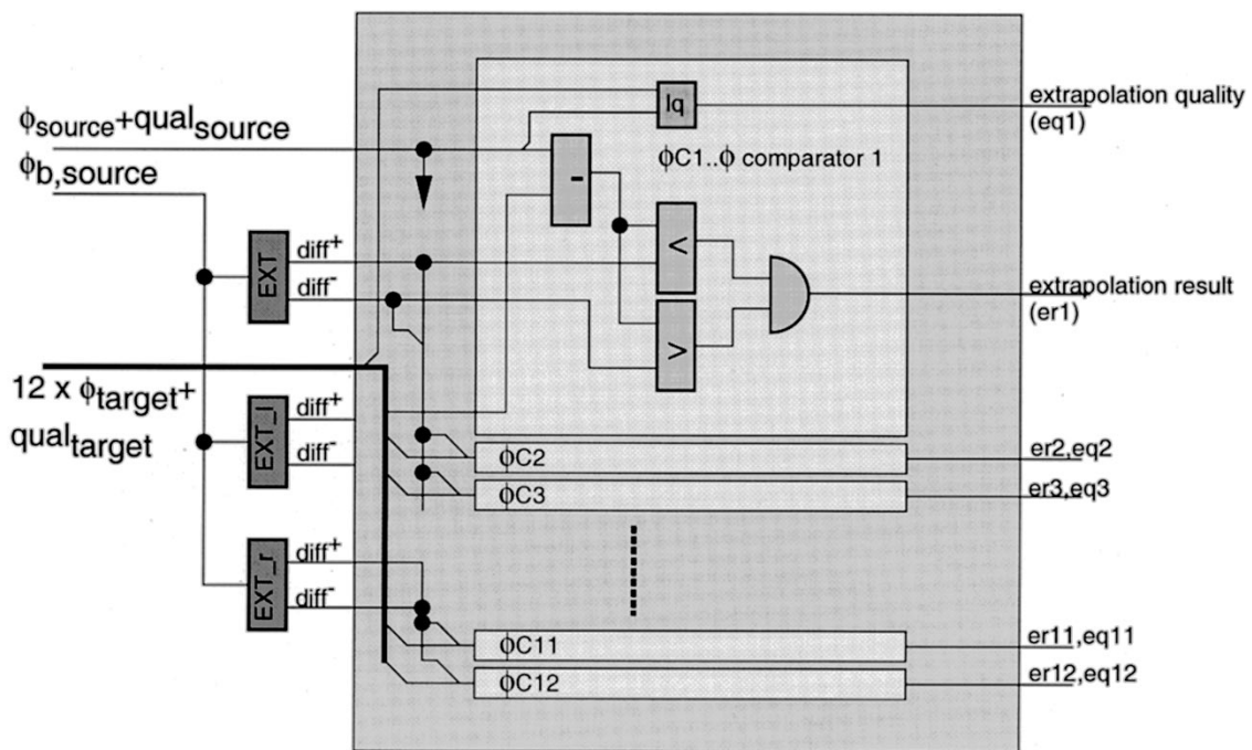
Fig. 17. Extrapolation unit extrapolates from one track segment and compares the extrapolated value to 12 target track segments. It outputs the extrapolation result ( er ) and the extrapolation quality ( eq ) for each comparison.
