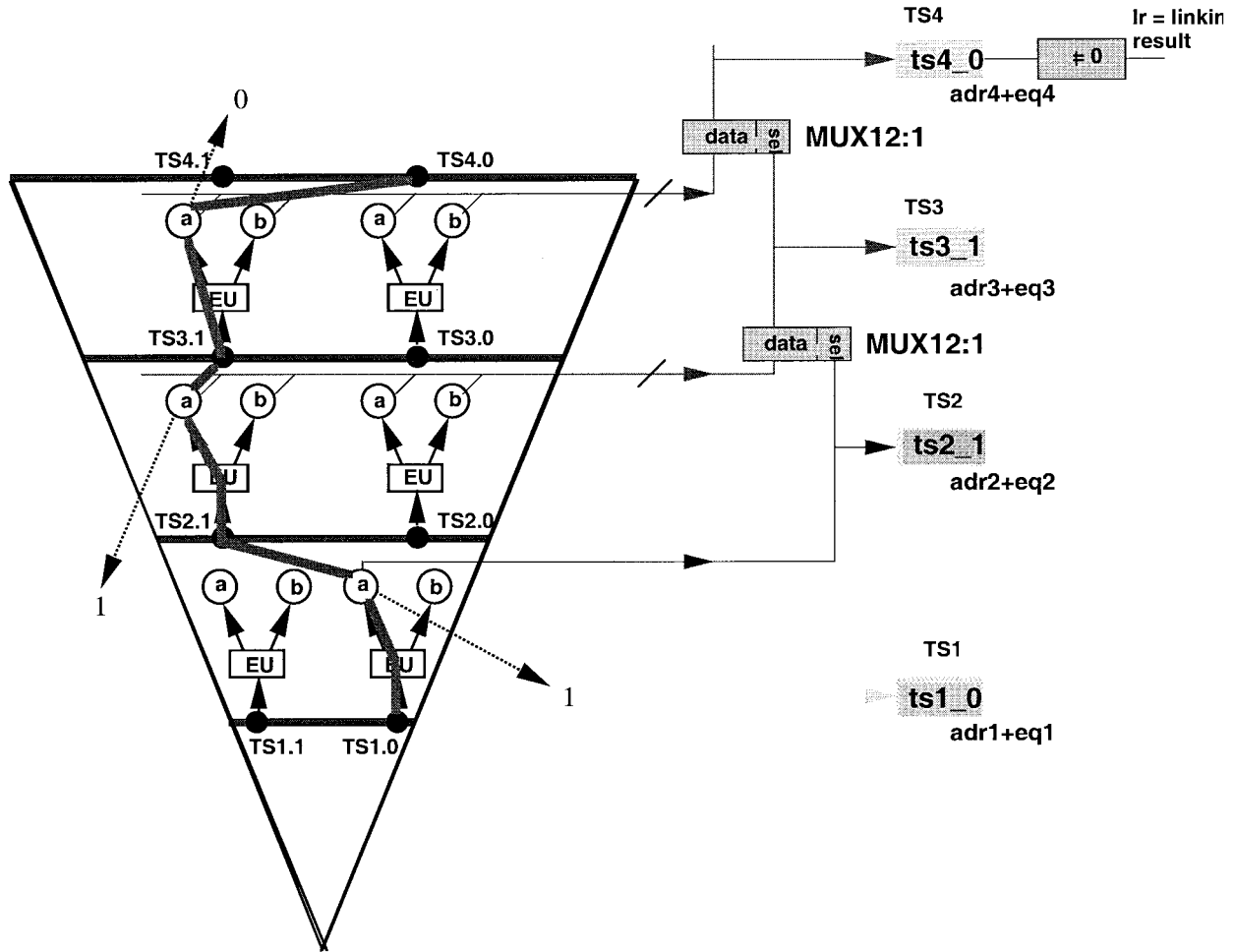
Fig. 18. Principle of track segment linker operation.
