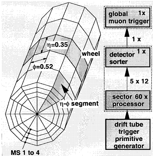
Fig. 14. Logical segmentation of the track finder processor.
