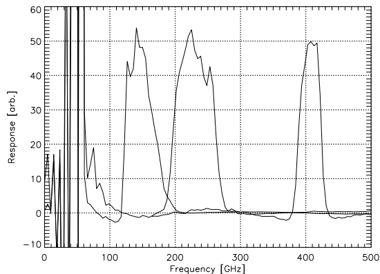
FIGURE 5. Spectral response of detector system. The data were obtained with a far-infrared Fourier spectrometer. The receiver was in flight configuration. The high noise below 100 GHz results from the measurement method and does not reflect detector response.
