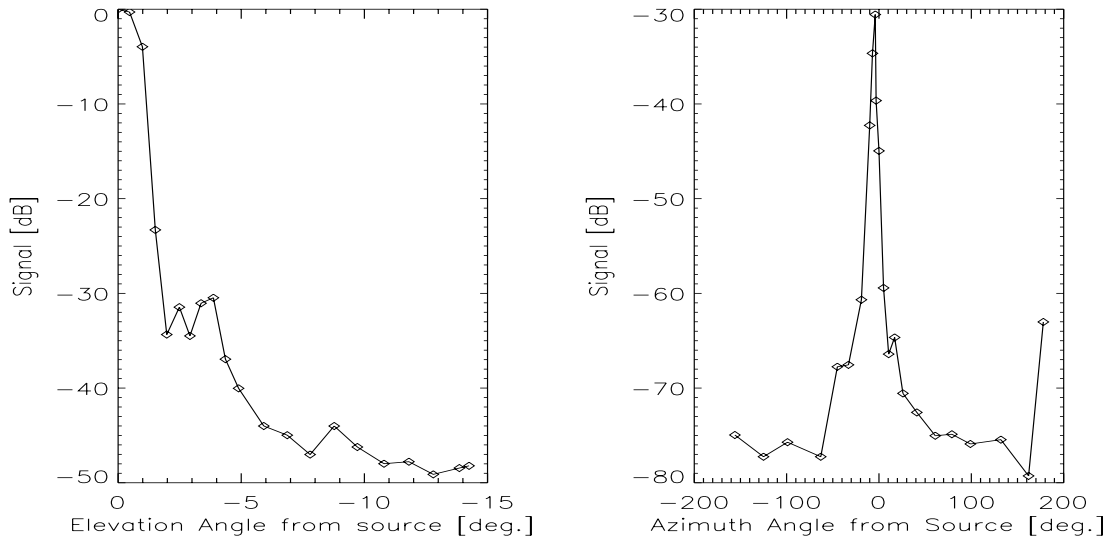
FIGURE 8. Sidelobe patterns for the MAXIMA telescope at 150 GHz. The near sidelobe pattern in elevation is at the left, and far sidelobe pattern in azimuth is at the right. Measurements were done with source on top of the NSBF highbay with a source elevation of 42^\circ . Adjustable attenuators were used on the source to keep the detectors in the linear regime. The azimuth measurements were done with the elevation \approx 2^\circ below the elevation of the source. This suppressed the main lobe during azimuth scan.
