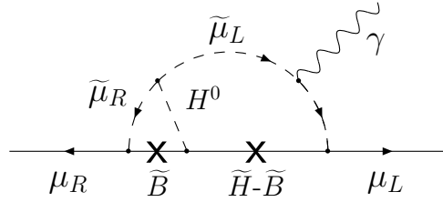
FIG. 15. Two-loop one-particle-irreducible contribution to the muon anomalous magnetic moment. In the heavy Higgs limit the one-loop sub-diagram on the left corresponds to the radiative Higgsino–scalar–fermion coupling of fig. 6. There are additional contributions from chirality conserving gaugino propagators.
