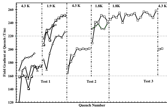
Figure 1: Training history of the three 70 mm single aperture quadrupoles: Q1 (diamonds), Q2 (triangles), Q3 (squares). Quenches were performed at the nominal ramp rate of 5 A/s. Starting from quench no. 4 of test 3, the fraction of energy dissipated in Q3 was increased to 100%. Horizontal dashed lines represent nominal operating gradients in the LHC: 160 T/m at 4.5 K and 220 T/m at 1.9 K. The short sample gradients are 200 T/m at 4.3 K and 260 T/m at 1.9 K.
