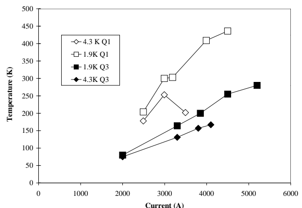
Figure 2: Peak temperatures in Q1 and Q3 at 4.3 K and 1.9 K. The overall error in peak temperature is \pm 15 K.
