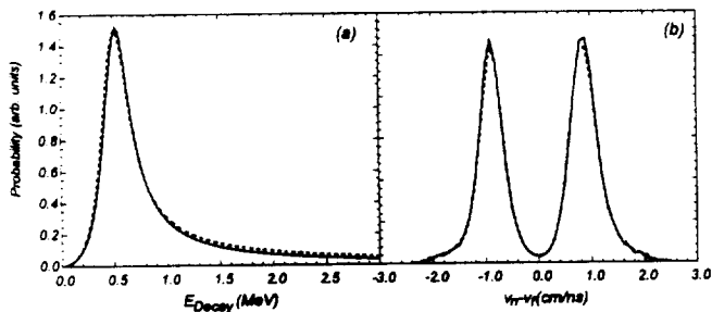
FIG. 5. Comparison of the energy (a) and the relative velocity (b) of the p -wave resonance calculated with the potential model and a calculation using a Breit-Wigner shape (solid) with energy and width parameters of Ref. [34] (dashed).
