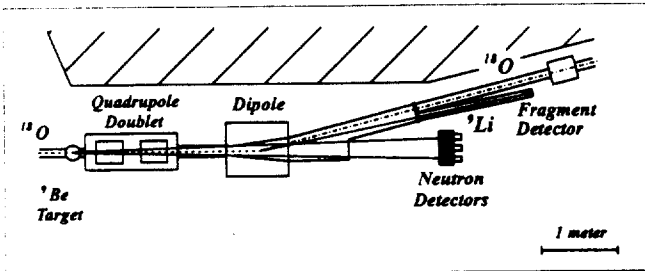
FIG. 1. Experimental Setup.
