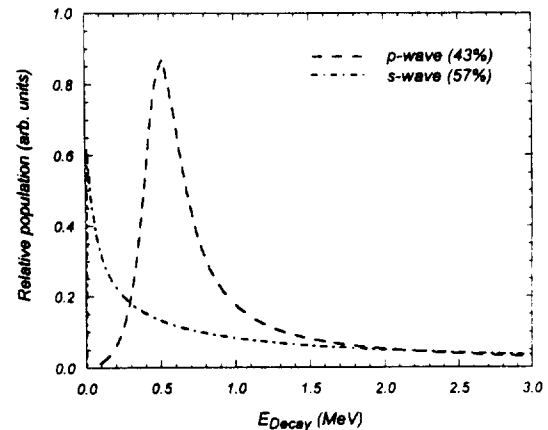
FIG. 6. Relative population of the s -wave (dot-dashed) and the p -wave (dashed) assuming the parameters from Figure 3.
