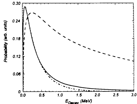
FIG. 8. Potential model calculations for a scattering length of a_s = -5 fm. For weakly bound neutrons (280 keV) the potential model (solid) and the parameterization of Ref. [9] (dot-dashed) are in good agreement. The energy distribution of initially more strongly bound neutrons (8 MeV) calculated with the potential model is substantially wider (dashed).
