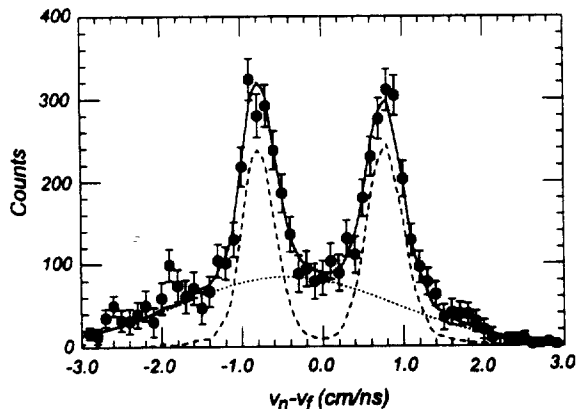
FIG. 2. Relative velocity spectrum of ^7\text{He} . The right and the left peak correspond to forward and backward emitted neutrons, respectively. The solid line is the result of Monte-Carlo simulations with the known values of the decay of ^7\text{He} ( E_{\text{decay}} = 450 keV, \Gamma_{\text{decay}} = 160 keV) (dashed) and an estimated background (dotted).
