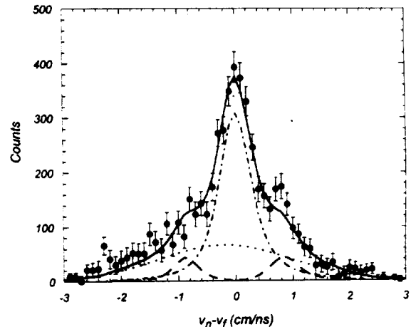
FIG. 3. Relative velocity spectrum of ^{10}\text{Li} . The Monte-Carlo simulations (solid) include contributions from an s -wave with a_s = -30 fm (dot-dashed), a p -wave at E_{\text{decay}} = 538 keV, \Gamma_{\text{decay}} = 358 keV (dashed) and an estimated background (dotted).
