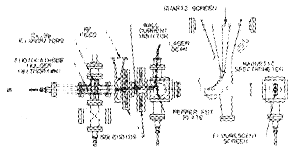
Fig. 1 Plan view of the photoinjector experiment
