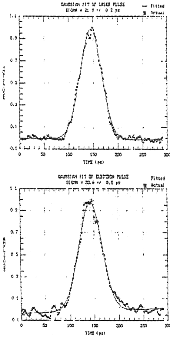
Fig 6 Digitized streak camera temporal profiles of the laser and photoinjector beams
