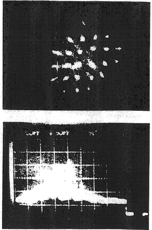
Fig. 7. (a) Pepper pot image 92 cm from a tantalum plate with 1217 \mu\text{m} diam holes on 2 mm centers; (b) a cut through one row of spots; the horizontal scale is 7.8 mm per 5 \mu\text{s}
