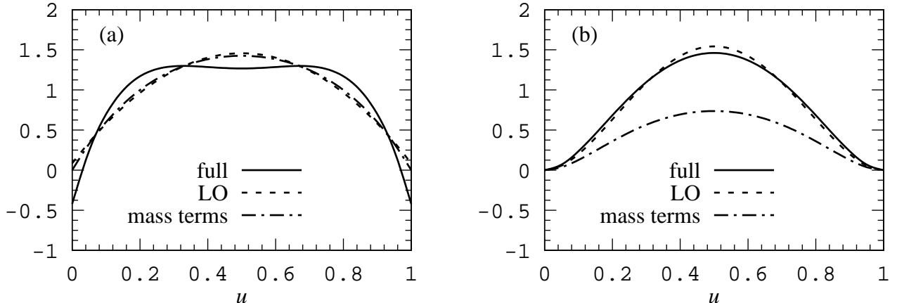
Figure 2: Two-particle twist-4 chiral-odd distribution amplitudes of the \rho meson: h_3 (a) and \mathbb{A}_T (b). LO means neglecting contributions of higher conformal spin for twist-3 and twist-4 operators and the mass terms correspond to retaining meson mass corrections only.
