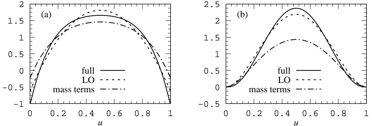
Figure 1: Two-particle twist-4 chiral-even distribution amplitudes of the \rho meson: g_3 (a) and \mathbb{A} (b). LO means neglecting contributions of higher conformal spin for twist-3 and twist-4 operators and the mass terms correspond to pure meson mass corrections.
