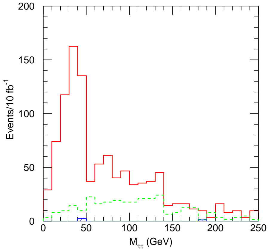
FIG. 4. Visible \tau\tau mass with 3-prong decays (solid), SUSY background estimate from \tau^{\pm}\tau^{\pm} (dashed), and SM background (shaded).
