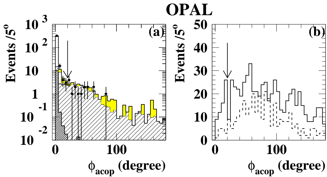
Figure 3: The distributions of the acoplanarity angle after cut (A3) for background (histograms) and data in (a), and for the \tilde{\tau}_1 \tilde{\tau}_1 predictions in (b). The conventions for the various histograms are the same as in Fig. 1.
