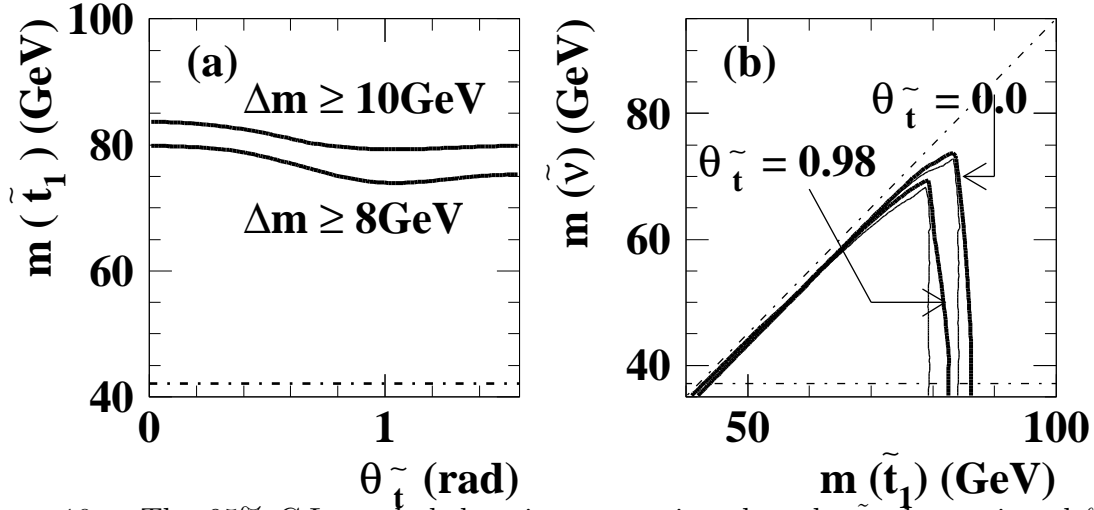
Figure 10: The 95% C.L. excluded regions assuming that the \tilde{t}_1 decays into b l \tilde{\nu} and that the branching fraction to each lepton flavour is the same. (a) The excluded regions in the (\theta_{\tilde{t}}, m_{\tilde{t}_1}) plane where the mass difference between the \tilde{t}_1 and the \tilde{\nu} is greater than 8 or 10 GeV. The dash-dotted straight line shows the kinematic limit for this decay, since a \tilde{\nu} lighter than 37.1 GeV has been excluded [34, 30]. (b) The excluded regions in the (m_{\tilde{t}_1}, m_{\tilde{\nu}}) plane, for a mixing angle of the \tilde{t}_1 assumed to be 0.0 and 0.98 rad. The solid lines show the actual limits, and the thin lines show the limits calculated only with the expected number of background events. The dash-dotted horizontal line shows the limit on m_{\tilde{\nu}} obtained at LEP1, and the dash-dotted diagonal line shows the kinematic limit for the \tilde{t}_1 \rightarrow b l \tilde{\nu} decay.
