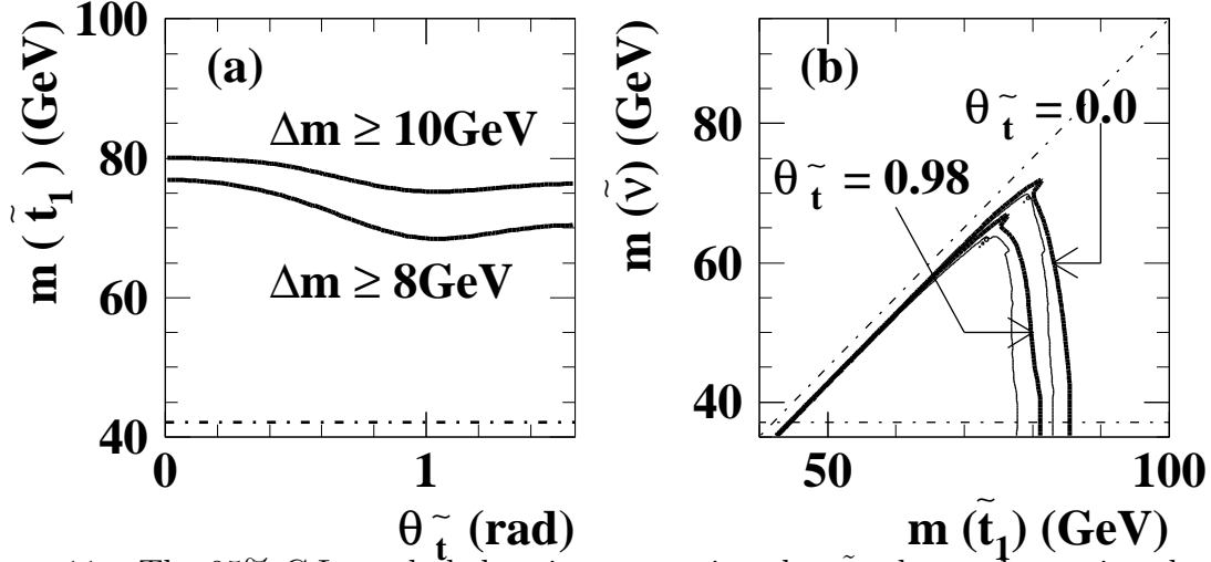
Figure 11: The 95% C.L. excluded regions assuming that \tilde{t}_1 always decays into b \tau \tilde{\nu}_\tau . (a) The excluded regions in the (\theta_{\tilde{t}}, m_{\tilde{t}_1}) plane where the mass difference between the \tilde{t}_1 and the \tilde{\nu}_\tau is greater than 8 or 10 GeV. The dash-dotted straight line shows the kinematic limit for this decay. (b) The excluded regions in the (m_{\tilde{t}_1}, m_{\tilde{\nu}}) plane, for a mixing angle of the \tilde{t}_1 assumed to be 0.0 and 0.98 rad. The solid lines show the actual limits, and the thin lines show the limits calculated only with the expected number of background events. The dash-dotted horizontal line shows the limit on m_{\tilde{\nu}} obtained at LEP1 [34, 30], and the dash-dotted diagonal line shows the kinematic limit for the \tilde{t}_1 \rightarrow b \tau \tilde{\nu} decay.
