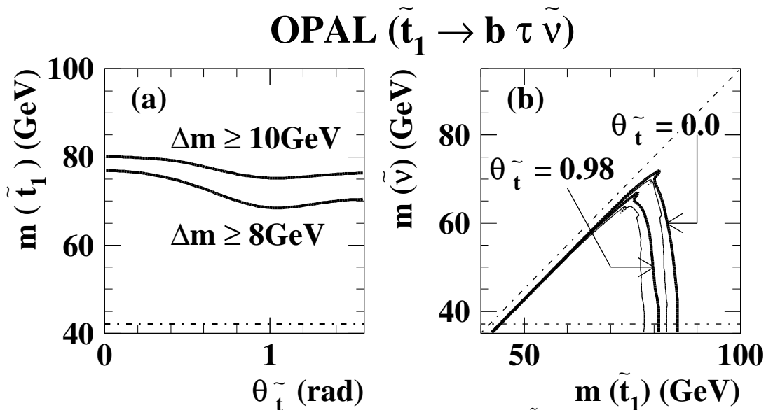
Figure 11: The 95% C.L. excluded regions assuming that \tilde{t}_1 always decays into b\tau\tilde{\nu}_\tau . (a) The excluded regions in the (\theta_{\tilde{t}}, m_{\tilde{t}_1}) plane where the mass difference between the \tilde{t}_1 and the \tilde{\nu}_\tau is greater than 8 or 10 GeV. The dash-dotted straight line shows the kinematic limit for this decay. (b) The excluded regions in the (m_{\tilde{t}_1}, m_{\tilde{\nu}}) plane, for a mixing angle of the \tilde{t}_1 assumed to be 0.0 and 0.98 rad. The solid lines show the actual limits, and the thin lines show the limits calculated only with the expected number of background events. The dash-dotted horizontal line shows the limit on m_{\tilde{\nu}} obtained at LEP1 [34, 30], and the dash-dotted diagonal line shows the kinematic limit for the \tilde{t}_1 \rightarrow b\tau\tilde{\nu} decay.
