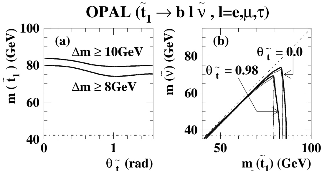
Figure 10: The 95% C.L. excluded regions assuming that the \tilde{t}_1 decays into bl\tilde{\nu} and that the branching fraction to each lepton flavour is the same. (a) The excluded regions in the (\theta_{\tilde{t}}, m_{\tilde{t}_1}) plane where the mass difference between the \tilde{t}_1 and the \tilde{\nu} is greater than 8 or 10 GeV. The dash-dotted straight line shows the kinematic limit for this decay, since a \tilde{\nu} lighter than 37.1 GeV has been excluded [34, 30]. (b) The excluded regions in the (m_{\tilde{t}_1}, m_{\tilde{\nu}}) plane, for a mixing angle of the \tilde{t}_1 assumed to be 0.0 and 0.98 rad. The solid lines show the actual limits, and the thin lines show the limits calculated only with the expected number of background events. The dash-dotted horizontal line shows the limit on m_{\tilde{\nu}} obtained at LEP1, and the dash-dotted diagonal line shows the kinematic limit for the \tilde{t}_1 \rightarrow bl\tilde{\nu} decay.
