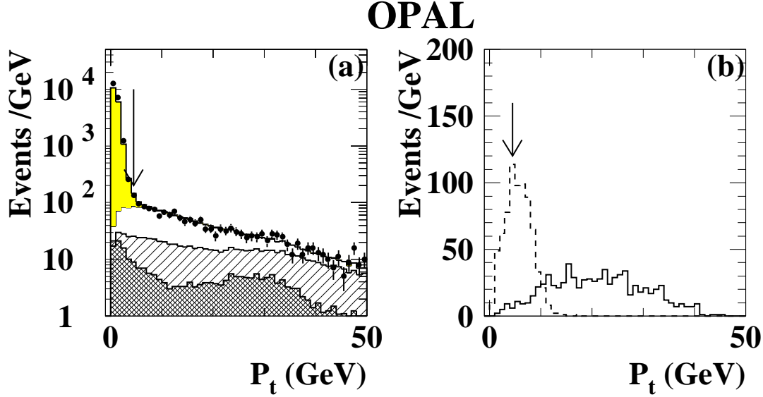
Figure 1: The distributions of P_t after cut (A1) for background (histograms) and data in (a), and for \tilde{t}_1\tilde{t}_1 predictions in (b). The arrows in these figures show the selection criteria. In (a) the distribution of the data is shown by the points with error bars. The predictions from background processes are also shown: dilepton events (cross-hatched area), two-photon processes (grey area), four-fermion processes (singly-hatched area), and multihadronic events (open area). (b) shows predictions for \tilde{t}_1\tilde{t}_1 in which \tilde{t}_1 decays into c\tilde{\chi}_1^0 . The continuous line histogram is for (m_{\tilde{t}_1}, m_{\tilde{\chi}_1^0}) = (80 \text{ GeV}, 60 \text{ GeV}) , and the dashed line is for (80 \text{ GeV}, 75 \text{ GeV}) , starting from 1000 generated events each.
