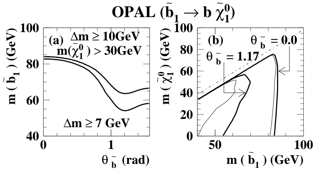
Figure 12: The 95% C.L. excluded regions assuming that the \tilde{b}_1 decays into b\tilde{\chi}_1^0 . (a) The excluded region in the (\theta_{\tilde{b}}, m_{\tilde{b}_1}) plane for a mass difference, \Delta m (= m_{\tilde{b}_1} - m_{\tilde{\chi}_1^0}) , \Delta m \geq 10 \text{ GeV} and \tilde{\chi}_1^0 is heavier than 30 GeV. The excluded region for \Delta m \geq 7 \text{ GeV} is also shown. (b) The excluded regions in the (m_{\tilde{b}_1}, m_{\tilde{\chi}_1^0}) plane, for a mixing angle of the \tilde{b}_1 assumed to be 0.0 and 1.17 rad. The solid lines show the actual limits, and the thin lines show the limits calculated only with the expected number of background events.
