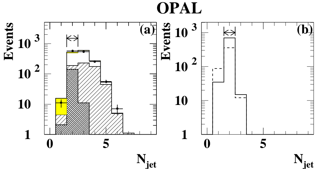
Figure 2: The distributions of the number of reconstructed jets after cut (A2): for background (histograms) and data in (a), and for \tilde{t}_1\tilde{t}_1 predictions in (b). The conventions for the various histograms are the same as in Fig. 1.
