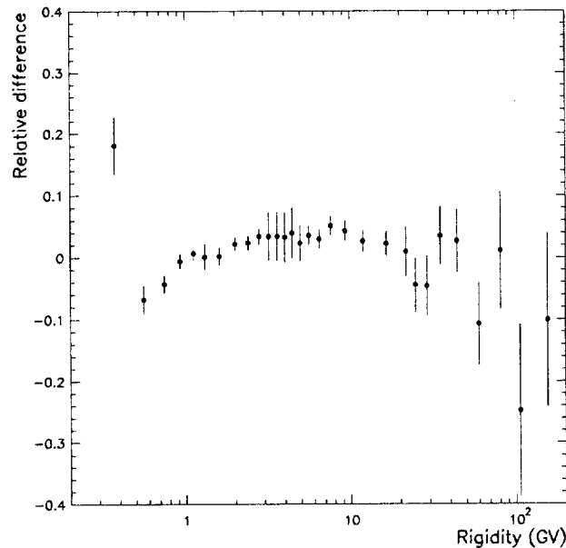
Figure 7 - The difference between the hydrogen nuclei spectrum at the spectrometer obtained with track fit of the complete tracking system information and with track fit of only drift chamber information, normalized with the spectrum of the complete tracking system, as a function of rigidity.
