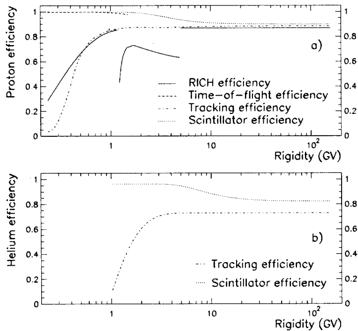
Figure 6 - Selection efficiencies as a function of rigidity for: a) hydrogen nuclei and b) helium nuclei.
