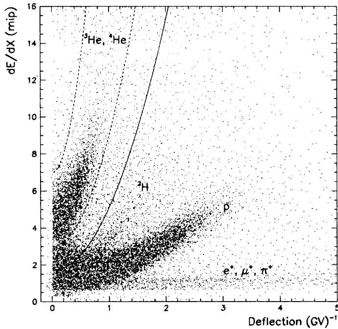
Figure 2 - Ionization loss in the top scintillator as a function of deflection in the magnetic field for all positive particles passing the tracking selection criteria ( \sim 648000 charge one and \sim 66000 charge two events). The solid and dashed lines show the selection criteria for Z=1 and Z=2 particles, respectively.
