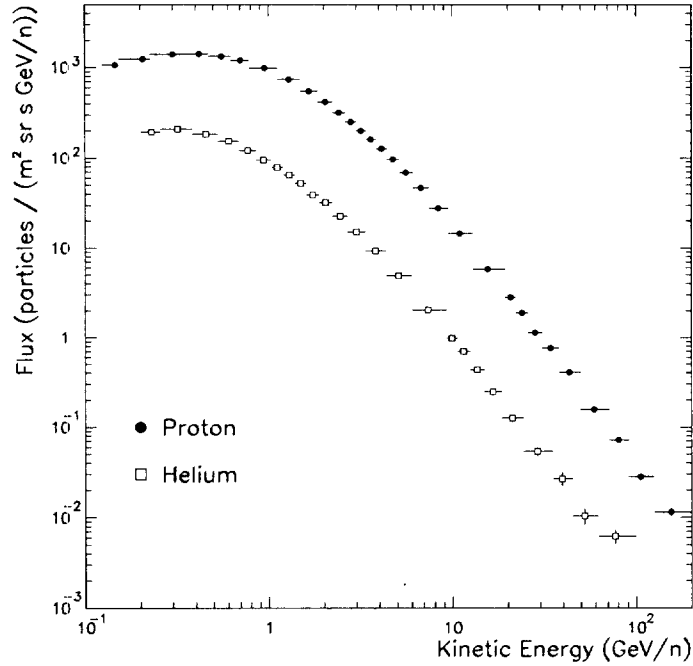
Figure 8 - Particle fluxes at the Top of the Atmosphere as a function of kinetic energy per nucleon: ● hydrogen nuclei spectrum; □ helium nuclei spectrum.
