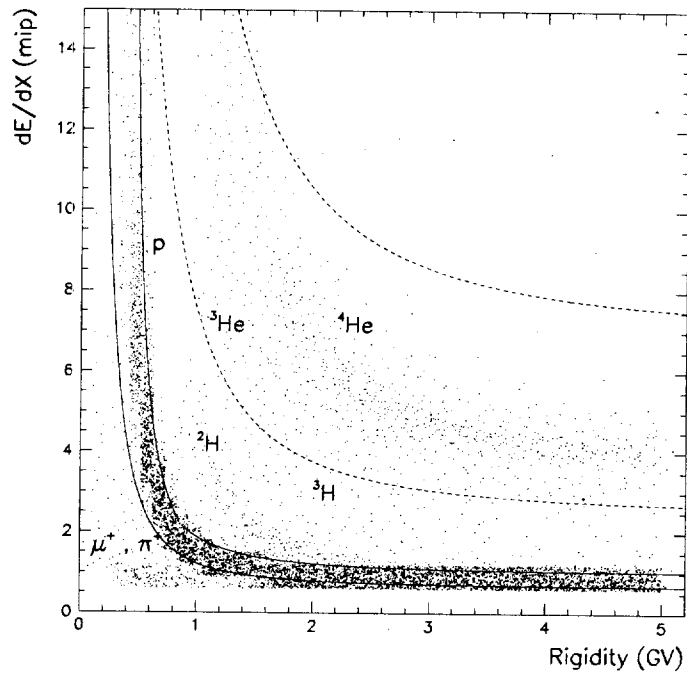
Figure 5 - Average energy loss in the calorimeter as a function of rigidity for all non-interacting (in the calorimeter) positive particles passing the tracking criteria ( \sim 282000 events of which \sim 268000 are protons and \sim 9000 are charge two particles). The proton and helium nuclei selection criteria are marked by the solid and dashed lines, respectively.
