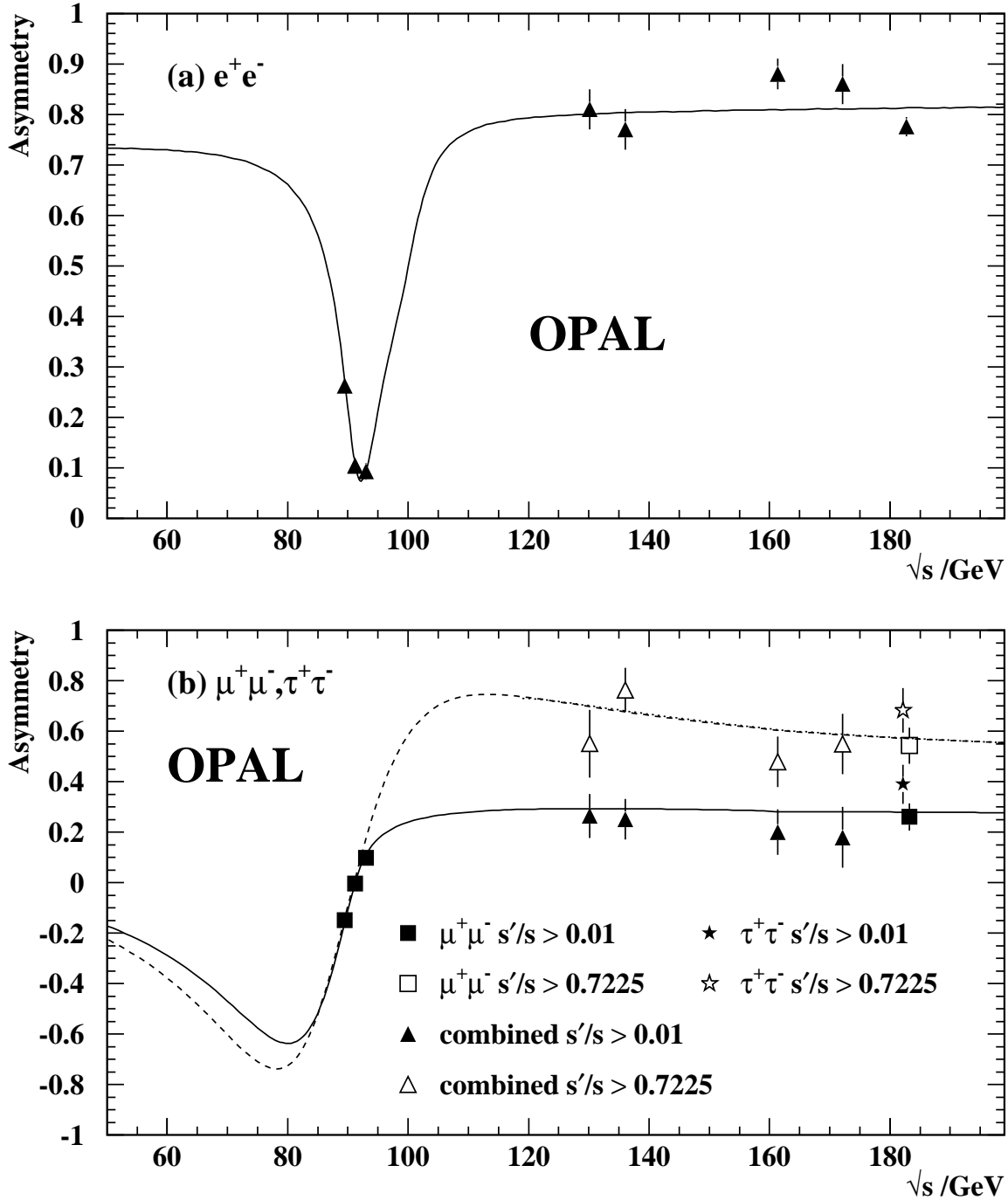
Figure 3: (a) Measured forward-backward asymmetry for electron pairs with |\cos\theta_e| < 0.7 and \theta_{\text{acol}} < 10^\circ , as a function of \sqrt{s} . The curve shows the prediction of ALIBABA. (b) Measured asymmetries for all ( s'/s > 0.01 ) and non-radiative ( s'/s > 0.7225 ) samples as functions of \sqrt{s} for \mu^+\mu^- and \tau^+\tau^- events. The curves show ZFITTER predictions for s'/s > 0.01 (solid) and s'/s > 0.7225 (dotted), as well as the Born-level expectation without QED radiative effects (dashed). The expectation for s'/s > 0.7225 lies very close to the Born curve, such that it appears indistinguishable on this plot.
