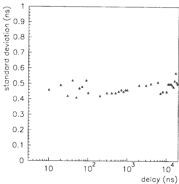
Figure 23: Time resolution in the 20 \mu s range.
