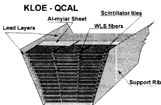
Figure 31: A QCAL module: the lead and scintillator tiles and the WLS fibers are clearly visible.
