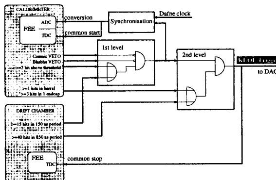
Figure 27: Architecture and conditions of the KLOE trigger system.
