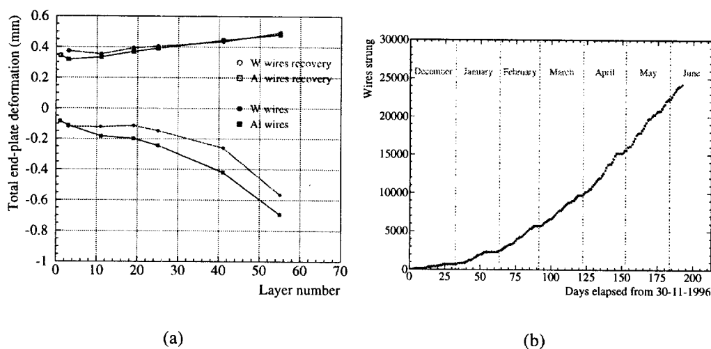
Figure 6: (a) The deformation of the end-plates and its recovery are monitored by measuring the mechanical tension on a sample of wires; (b) The integrated “stringosity”, defined as total number of wires strung as a function of the elapsed time of stringing.
