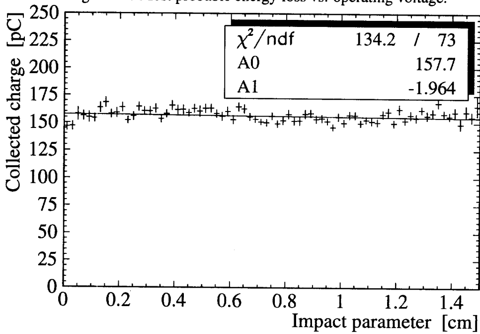
Figure 15: Collected charge as a function of the track's impact parameter.
