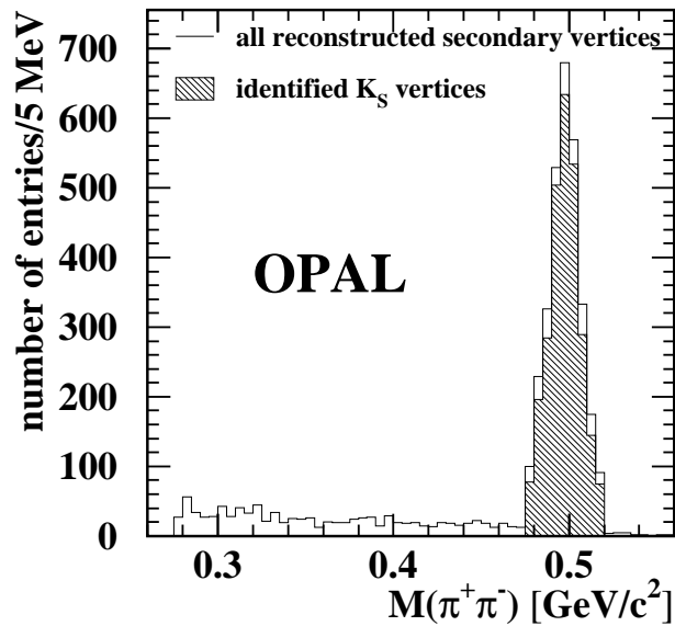
Figure 2: Distribution of the \pi^+\pi^- invariant mass M for all identified secondary vertices in the selected events before (open histogram) and after (hatched histogram) applying the cut |M(\pi^+\pi^-) - 0.4977 \text{ GeV}/c^2| < 0.02 \text{ GeV}/c^2 and the dE/dx cuts used to identify K_S^0 \rightarrow \pi^+\pi^- vertices.
