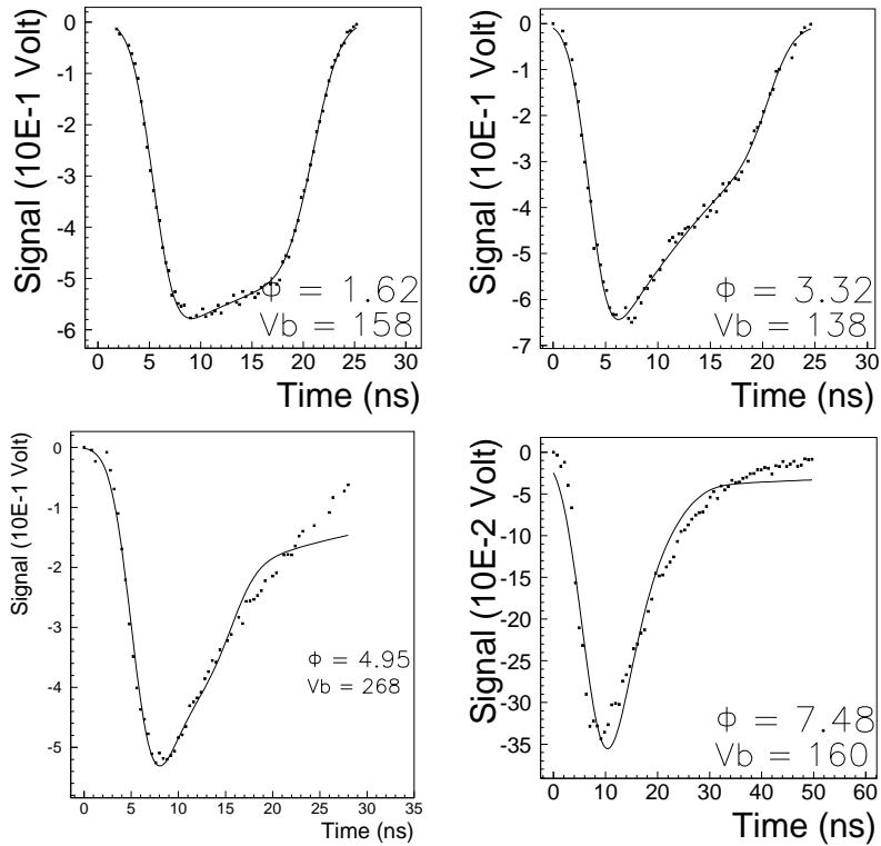
Figure 15: Fits for a p^+ - n - p - n^+ diode with a double junction (resulting from the introduction of the 15 \mu\text{m} n-type junction on the p^+ side after inversion) for the M18 detector, with \alpha particles on the front side (alpha front) and on the rear side (alpha back) for successive levels of fluence \Phi = 1.62 \times 10^{13} p/cm 2 up to \Phi = 7.5 \times 10^{13} p/cm 2 ( \Phi in 10^{13} p/cm 2 , V_b the applied voltage in volts)
