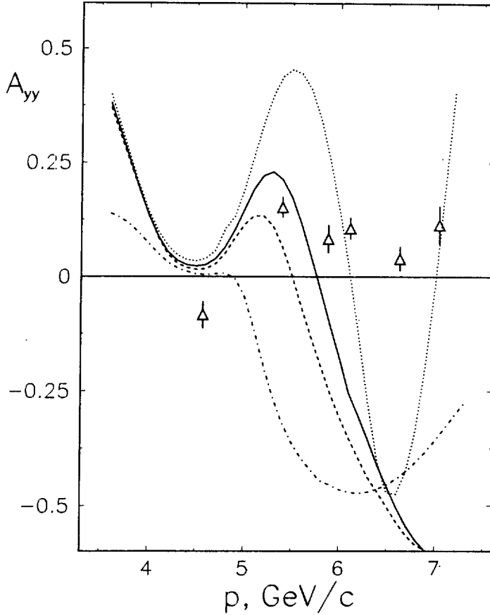
Fig.3. A_{yy} data as compared with the predictions of the hard scattering model [25] using different conventional DWFs. The solid, long-dashed, dotted and dash-dotted lines represent the results of calculations with Paris [30], RSC [31], Bonn [32] and Moscow [33] DWFs, respectively.
