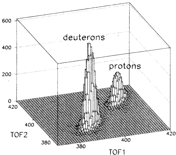
Fig.2. Two-dimensional plot of 2 different TOF over a baseline of \sim 28\text{ m} at a beam line momentum \sim 7.0\text{ GeV}/c . The deuterons are in part suppressed by the Čerenkov counter.
