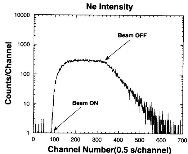
Figure 1: Time spectrum of ^{19}\text{Ne}^{2+} intensity measured by a Ge detector at the secondary target position. The intensity of primary protons was 100 nA.
