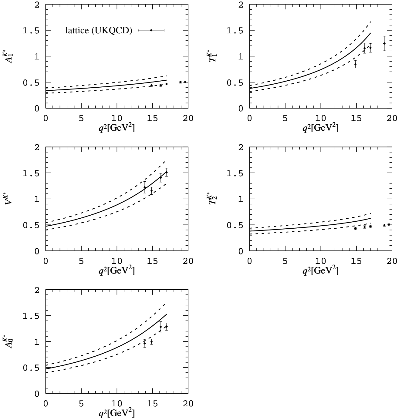
Figure 7: Comparison of the light-cone sum-rule predictions for the B \rightarrow K^* form factors with lattice calculations [22, 23]. Lattice errors are statistical only. The dashed curves show the 15% uncertainty range.
