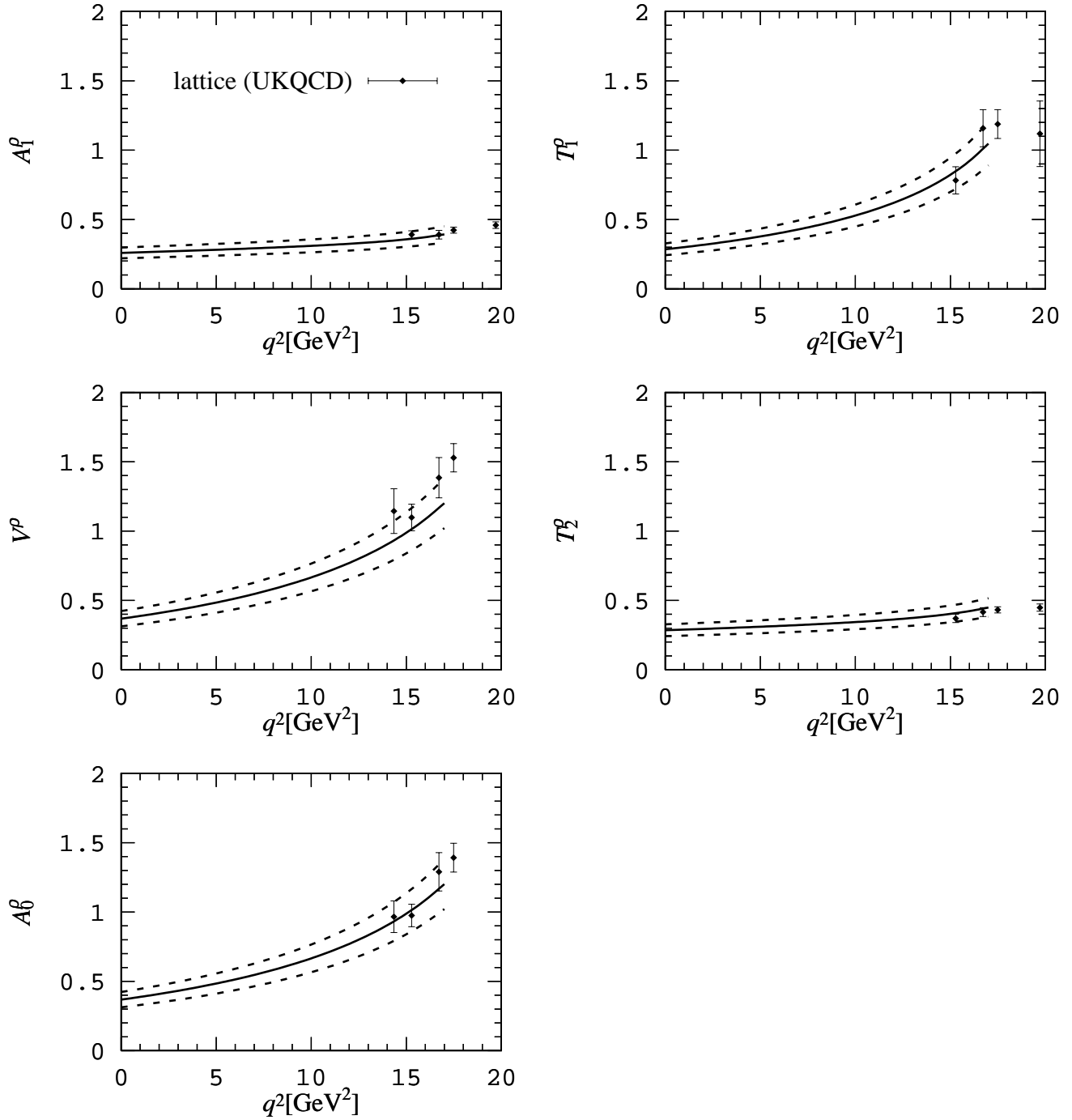
Figure 6: Comparison of the light-cone sum-rule predictions for the B \rightarrow \rho form factors with lattice calculations [22, 23]. Lattice errors are statistical only. The dashed curves show the 15% uncertainty range.
