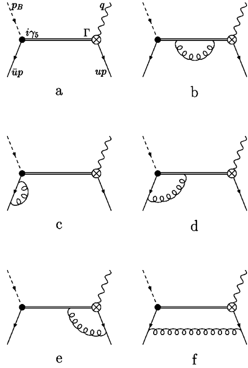
FIG. 1. The leading order diagram (a) and one-loop radiative corrections (b)–(f).
