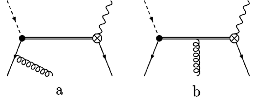
FIG. 2. The higher-twist contributions.
