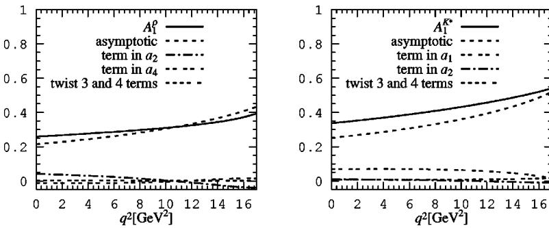
FIG. 5. Separate contributions to the form factors A_1^\rho and A_1^{K^*} .
