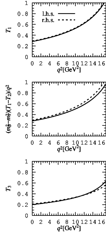
FIG. 9. Isgur-Wise relations (4.4)–(4.6) for B \rightarrow \rho transitions. Renormalization scale is \mu = m_b . Solid and dashed curves correspond to expressions appearing on the LHS and RHS, respectively.
