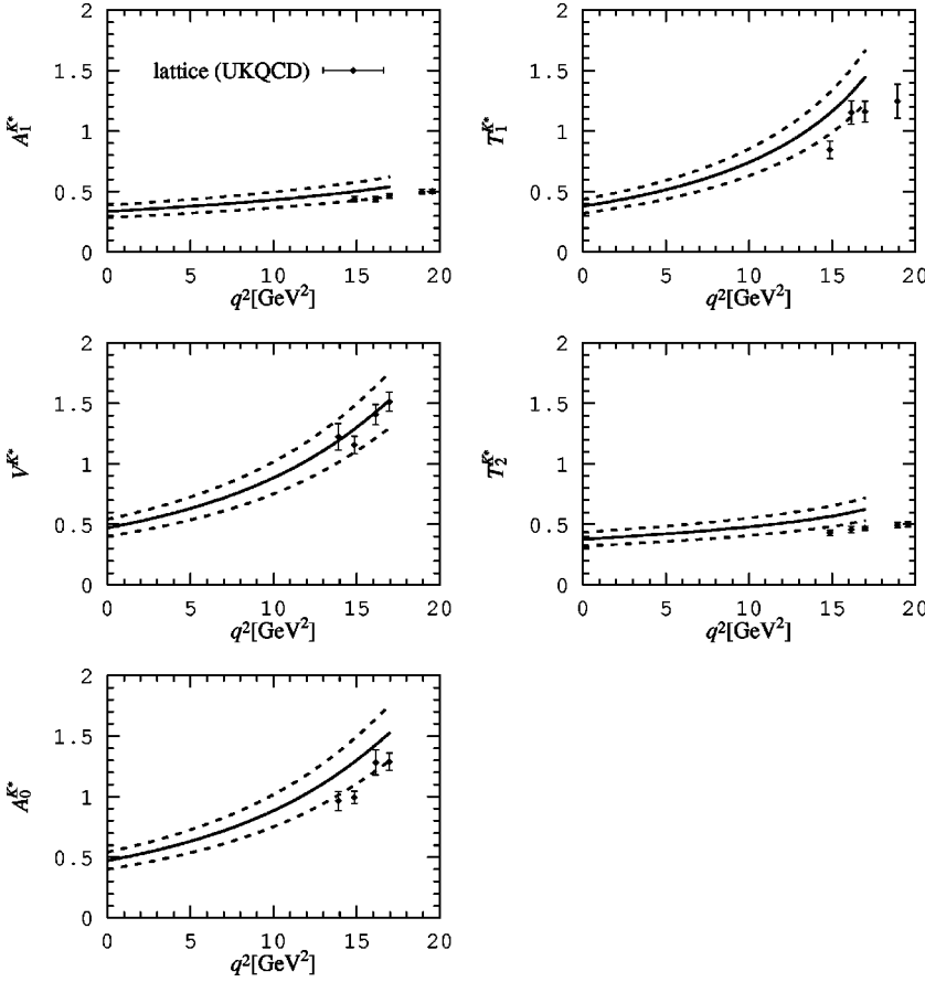
FIG. 7. Comparison of the light-cone sum rule predictions for the B \rightarrow K^* form factors with lattice calculations [25,26]. Lattice errors are statistical only. The dashed curves show the 15% uncertainty range.
