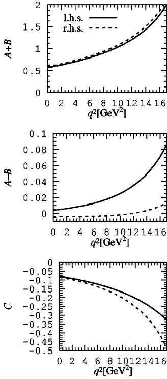
FIG. 8. Isgur-Wise relations (4.1)–(4.3) for B \rightarrow \rho transitions. Renormalization scale is \mu = m_b . Solid and dashed curves correspond to expressions appearing on the LHS and RHS, respectively.
