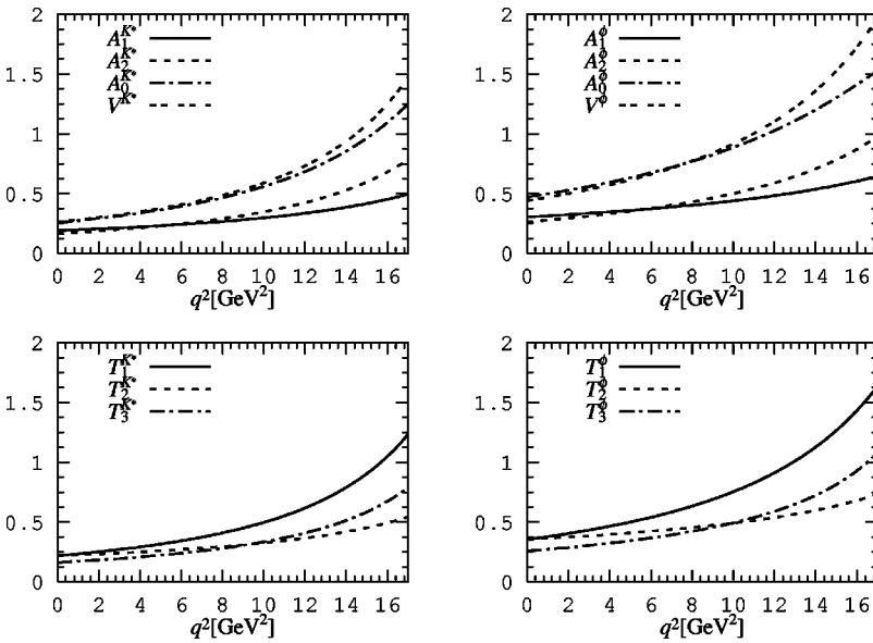
FIG. 4. Light-cone sum rule results for B_s \rightarrow vector meson form factors. The renormalization scale for T_i is \mu = m_b = 4.8 GeV. Further parameters are m_b = 4.8 GeV, s_0 = 34.5 GeV 2 , M^2 = 6 GeV 2 .
