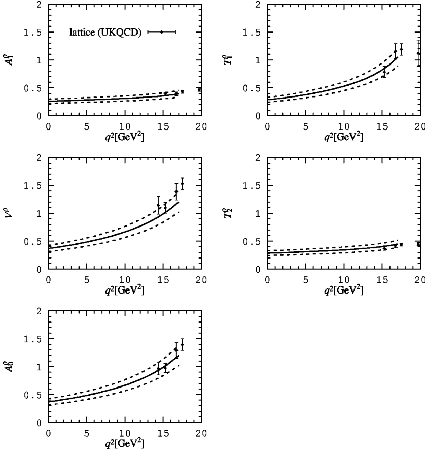
FIG. 6. Comparison of the light-cone sum rule predictions for the B \rightarrow \rho form factors with lattice calculations [25,26]. Lattice errors are statistical only. The dashed curves show the 15% uncertainty range.
