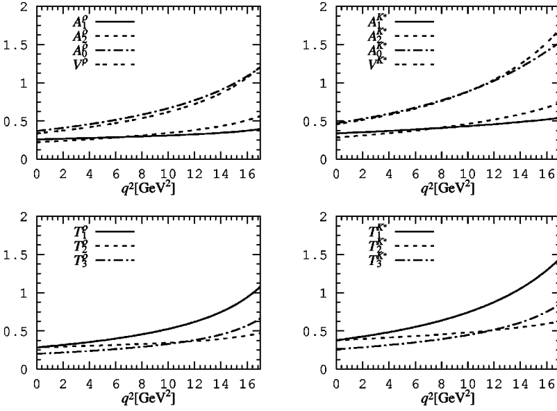
FIG. 3. Light-cone sum rule results for B_{u,d} \rightarrow vector meson form factors. The renormalization scale for T_i is \mu = m_b = 4.8 GeV. Further parameters are m_b = 4.8 GeV, s_0 = 33.5 GeV 2 , M^2 = 6 GeV 2 .
