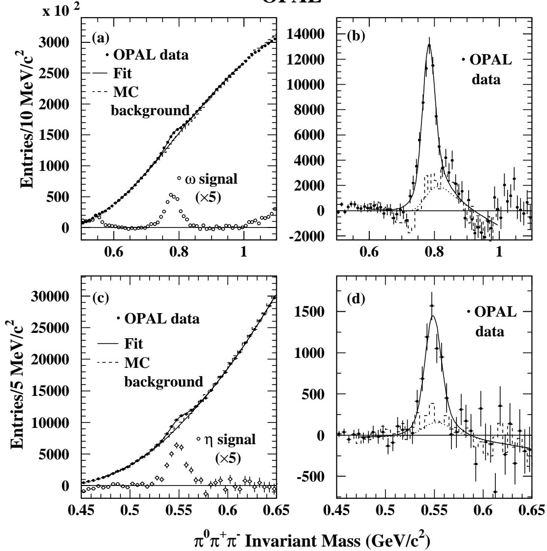
Figure 11: Fits to the invariant mass distribution of \pi^0\pi^+\pi^- combinations, for a cut of \tilde{G}_{\gamma\gamma}(m) > 0.3 . The points represent the OPAL data and the full curves the fit to the data. The dashed histograms correspond to the background evaluated using the Monte Carlo distributions. Fig. (a) and (c): fits in the region of the \omega and the \eta , respectively. The signal extracted from the fit to the data, multiplied by a factor 5 for clarity, is shown by the open circles. Fig. (b) and (d): the points are the components proportional to \lambda (see section 6.4) extracted from the data in the region of the \omega and the \eta , respectively. The full curves are the fits to the data. The dashed histogram is the simulated background, including partially reconstructed mesons which appear as a bump close to the signal peak. The dotted curves are the contributions from partial reconstructions included in the fit.
