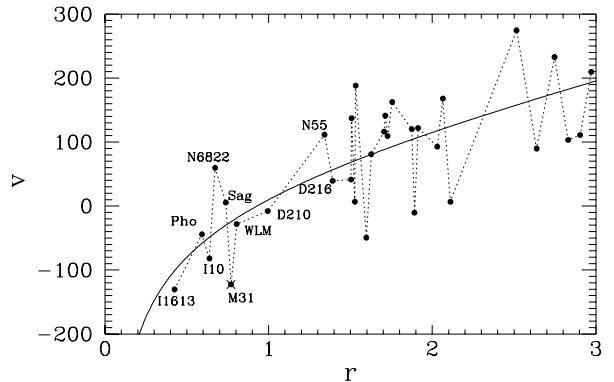
Fig. 2.— Phase space for the sample of nearby galaxies derived under the assumption of infall to the center of mass of the Milky Way – M31 system. The distance ( r ) from the center of mass is in Mpc, the infall velocity ( v ) is in km/s. For M31, r and v are the distance and the velocity relative to the Galaxy. The best fit infall trajectory, corresponding to R = 0.93 Mpc and h = 0.69 , is shown by the solid line.
