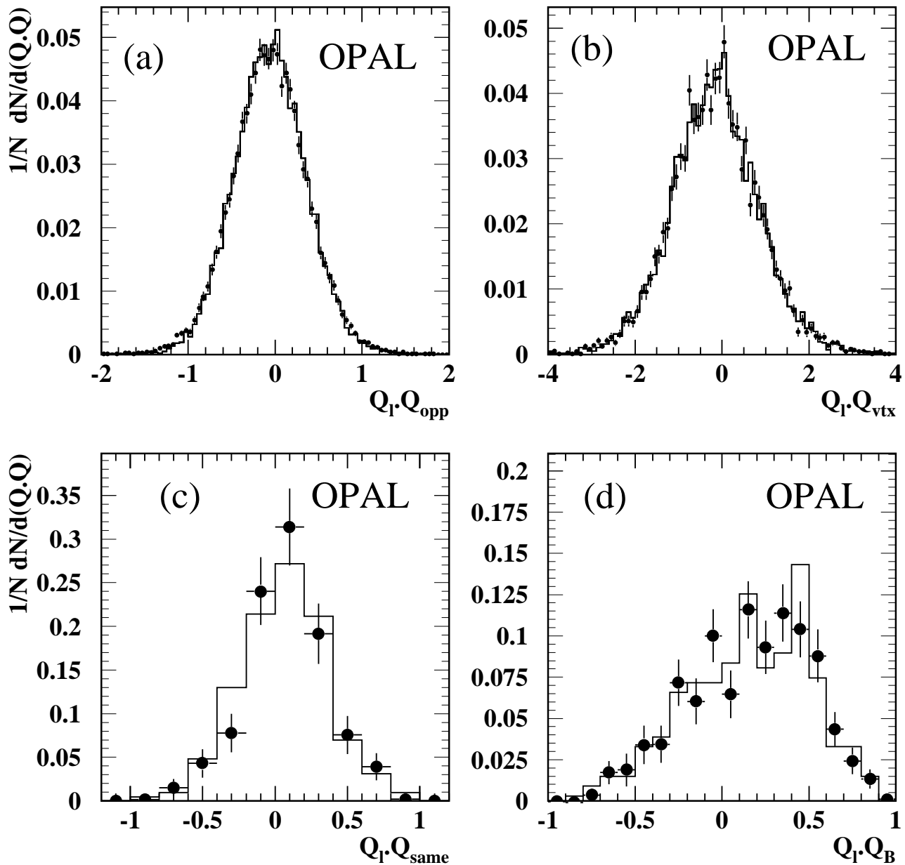
Figure 2: The distribution of the product of the lepton charge Q_l and (a) the Q_{\text{opp}}^{\kappa=0.5} jet charge, (b) the Q_{\text{vtx}} vertex charge, (c) the Q_{\text{same}}^{\kappa=0.4} jet charge and (d) the Q_B tagging variable. Distributions (a) and (b) are taken from an inclusive lepton sample, whilst distributions (c) and (d) are taken from a B^0 \rightarrow D^{*\pm} \ell sample, only including events with reconstructed proper time t_{\text{rec}} < 2 ps. The data are shown as points and the Monte Carlo predictions as histograms.
