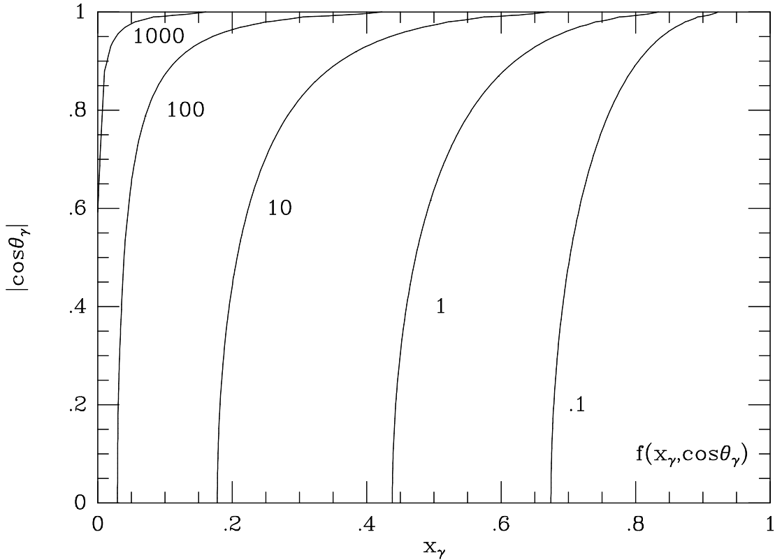
Figure 5: Contours of the function f of eq. (25) in the (x_\gamma, |\cos\theta_\gamma|) -plane.
