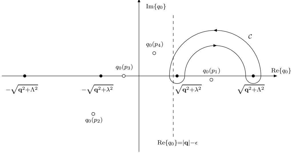
Figure 5: Illustration of the contour \mathcal{C} of (3.17) in the complex q_0 plane. The open circles indicate the “particle poles” located at q_0(p_i) = (2\mathbf{q}p_i - p_i^2 + m_i^2)/(2p_{i0}) .
