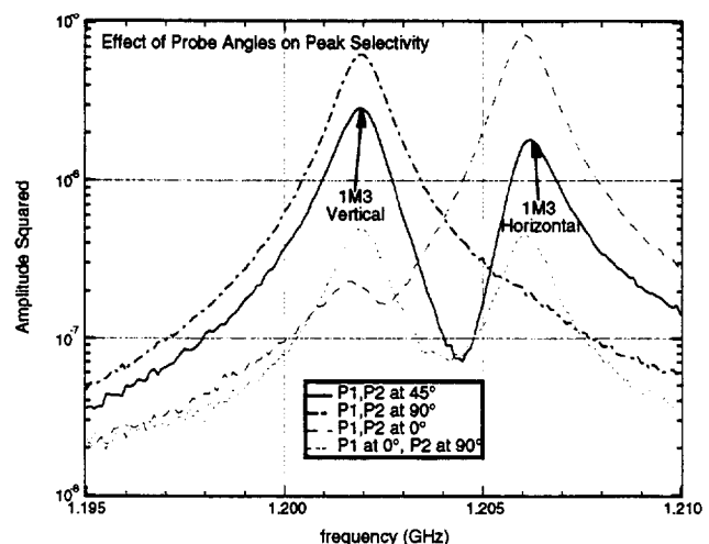
FIG. 3. Effect of probe angle on relative amplitudes of members of the 1M3 dipole pair.
