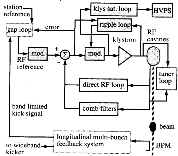
Fig. 2. Block diagram of RF feedback loops used in the PEP-II low-level RF system. Multi-cavities not shown for simplicity.
