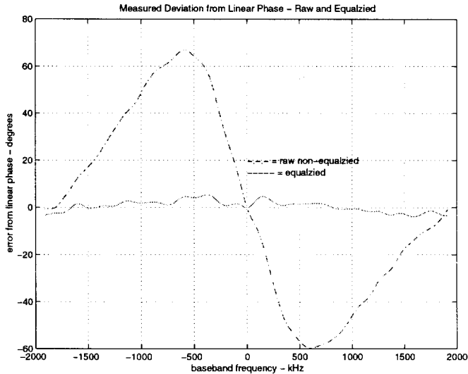
Fig. 4. Measured response of system without/with equalization.
