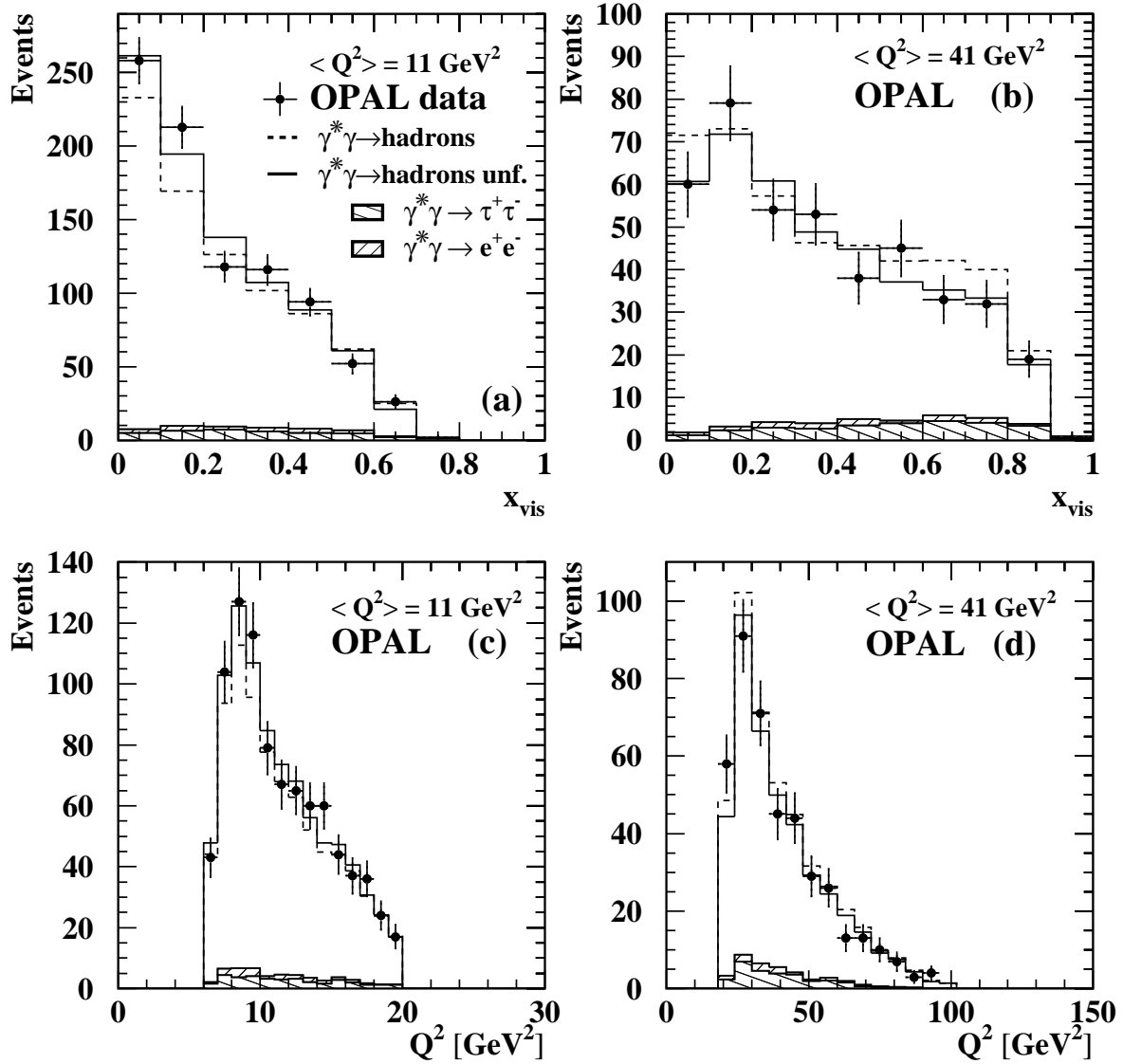
Figure 2: The x_{\text{vis}} , (a) and (b), and Q^2 , (c) and (d), distribution of the SW and FD samples for the data taken at \sqrt{s_{ee}} = 161 - 172 GeV. The dashed histogram, \gamma^*\gamma \rightarrow \text{hadrons} , shows the events from the HERWIG Monte Carlo, using the GRV parametrisation and the standard cuts (the reference sample), with the background added, before the unfolding; the solid histogram, \gamma^*\gamma \rightarrow \text{hadrons unf.} , shows the same quantity, but reweighted based on the result of the unfolding. The background events from the reactions \gamma^*\gamma \rightarrow \tau^+\tau^- and \gamma^*\gamma \rightarrow e^+e^- are also shown separately at the bottom of the figure. All errors shown are statistical only.
