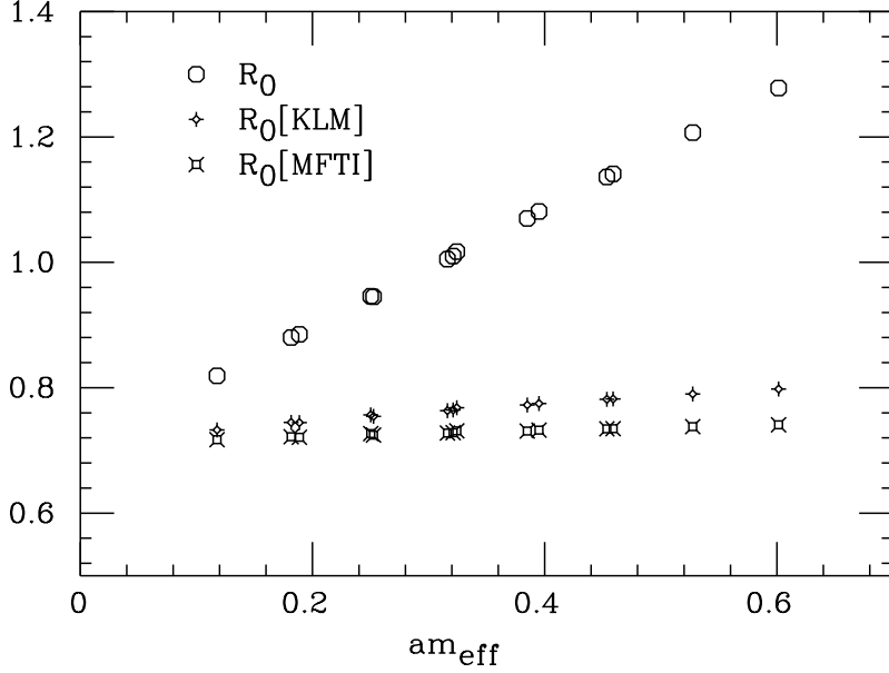
Figure 1: The various ratios R_0 , defined in eqs. (122), (123) and (124) for Wilson fermions, as functions of the effective quark mass.
