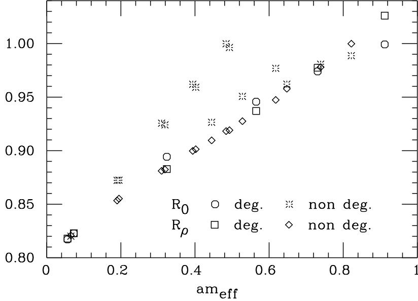
Figure 3: The ratios R_0 and R_\rho , for Clover fermions, as a function of the effective quark mass. We distinguish between the cases of degenerate and non-degenerate quarks in the current.
