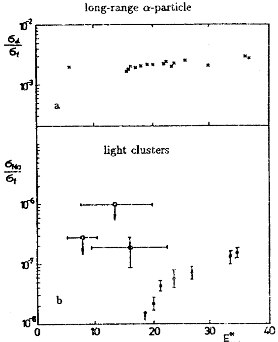
Figure 3: Excitation function for the ternary fission relative probability plotted: a) by data compiled in ref. 4 for long-range \alpha -particle emission and b) for ^{24}\text{Na} production by the results of ref. 7 - \circ , ref. 8 - \blacksquare , and present experiment - \square .
