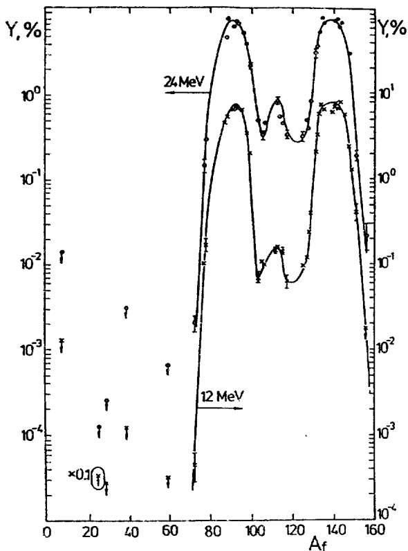
Figure 1: Final fragment mass-distributions of the bremsstrahlung-induced 232 Th fission.
