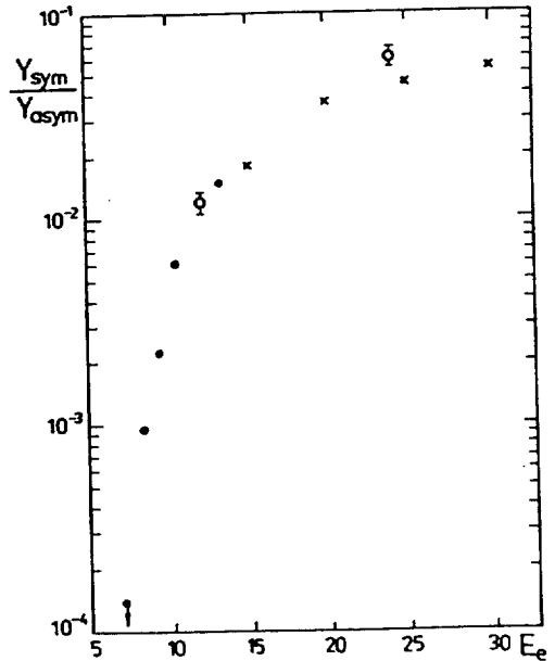
Figure 2: Symmetric-to-asymmetric modes abundance ratio as a function of E_c as it was measured in ref. 1 - •, ref. 3 - × and in present experiment - o.
