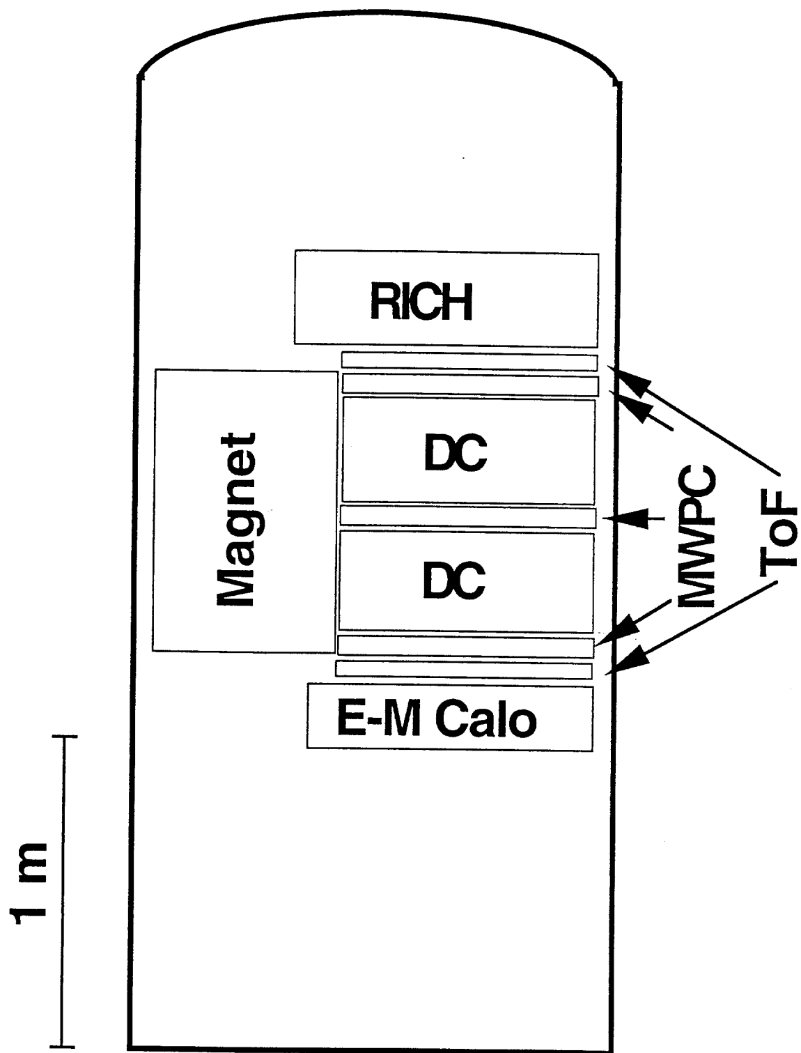
Fig. 1.— Schematic view of the CAPRICE apparatus.
