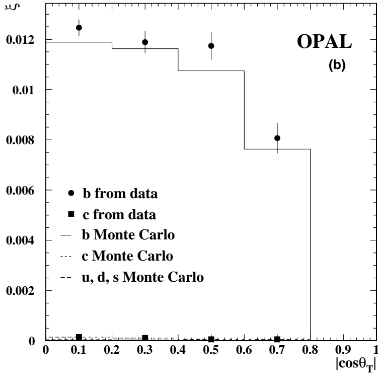
Figure 3: The fitted (a) lifetime tagged hemisphere and (b) q_{vtx} hemisphere tagging efficiencies for each |\cos\theta_T| bin. The histograms are the corresponding Monte Carlo quantities. Any discrepancy between the data and Monte Carlo b hemisphere efficiencies has no effect on the measurement as the values obtained from the data were used.
