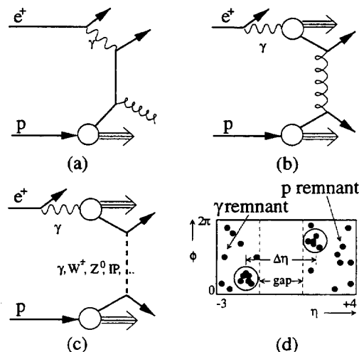
Figure 4: Feynman diagrams of LO processes in hard photoproduction: (a) and (b) are examples of direct and resolved contributions; (c) shows a color singlet exchange diagram and (d) shows how an event of the type displayed in (c) would appear in \eta - \phi space.
