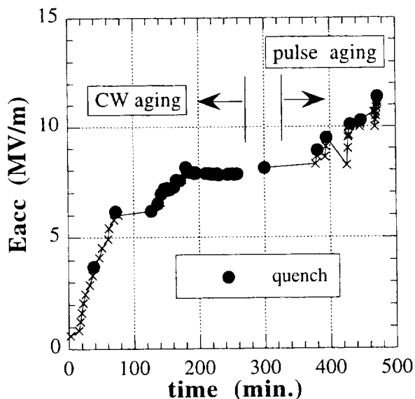
Figure: 2 Aging process in horizontal cold test.
