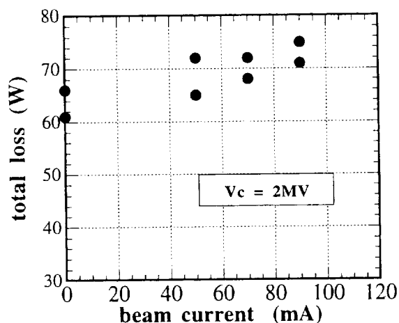
Figure: 4 Total loss measured by Lhe consumption at 2MV. The loss increases as the beam current.
