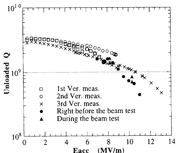
Figure: 3 The Q vs accelerating gradient (Eacc).
