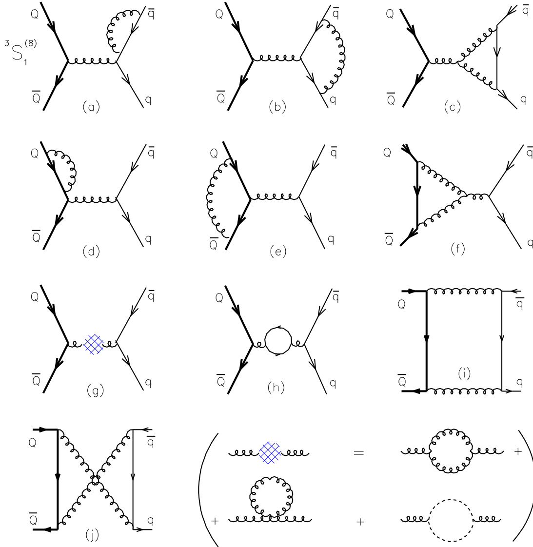
Figure 1: Virtual Feynman diagrams contributing to the process Q\bar{Q} [{}^3S_1^{(8)}] \rightarrow q\bar{q}
