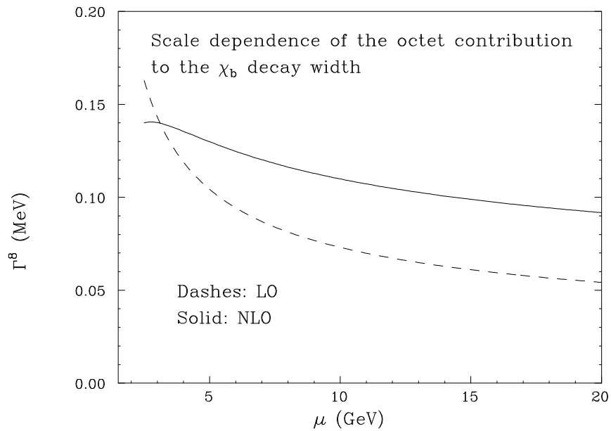
Figure 3: Same as fig. 2 but for \chi_b
