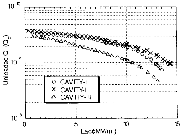
Fig.6: Q vs Eacc at vertical cold tests.
