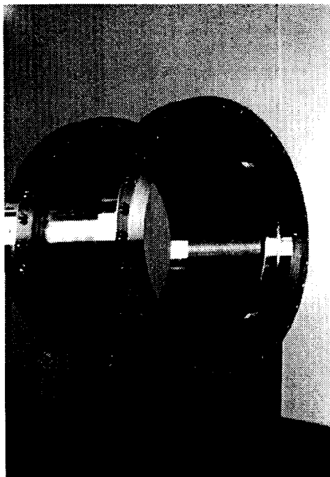
Fig.8: Full size model of ferrite damper. The powder of IB-004 ferrite was sintered and bonded on a Cu pipe by HIPping.
