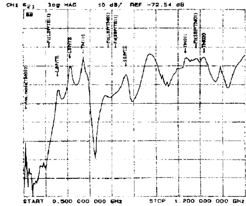
Fig.4: HOMs of an A1 model cavity with ferrite dampers.
