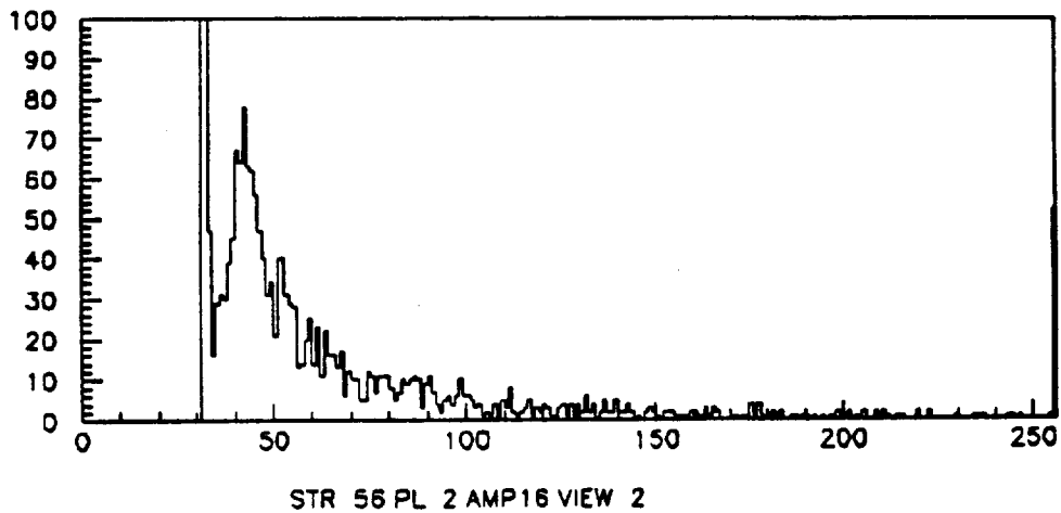
Figure 10 – Histogram of the energy deposited into two different strips. Counts are in arbitrary units while abscissa is in ADC channels. The saturation on the last (256th) ADC channel is also visible.
