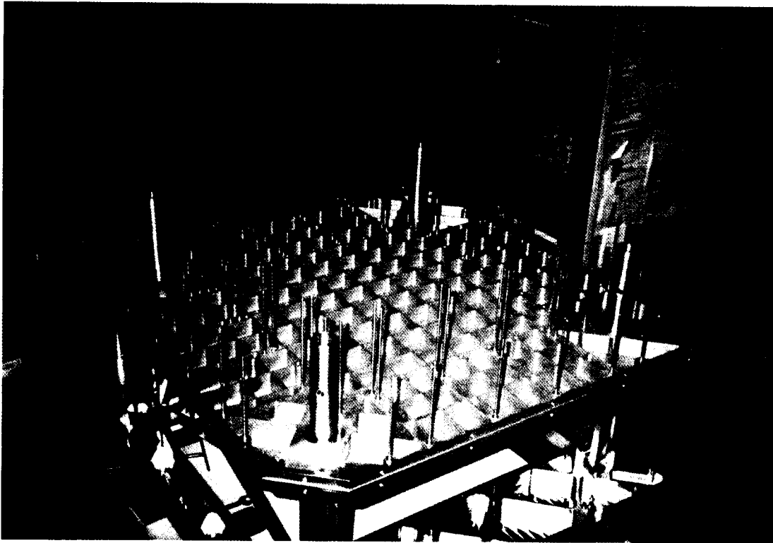
Figure 8 – Photograph of the bare mechanical structure showing the honeycomb base-plate with its four steel posts and all the threaded columns for the assembly of the planes (silicon and tungsten) and of the front-end boards.
