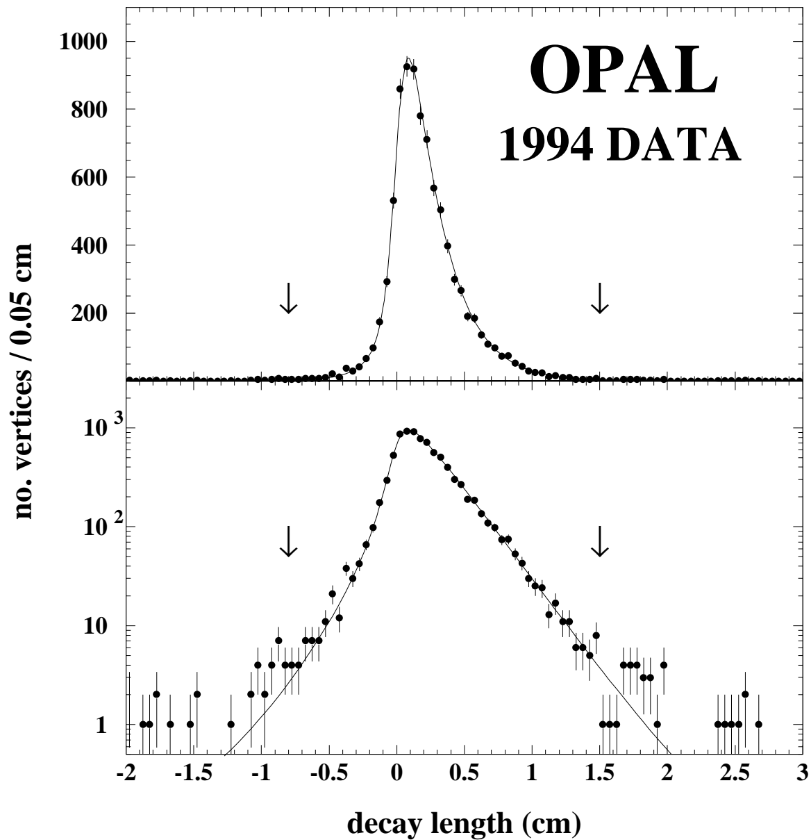
Figure 2: The decay length distribution for selected vertices. The result of the decay length fit is shown as the smooth curve superimposed on the plot. The lifetime was determined within the range of decay lengths delimited by the arrows.
