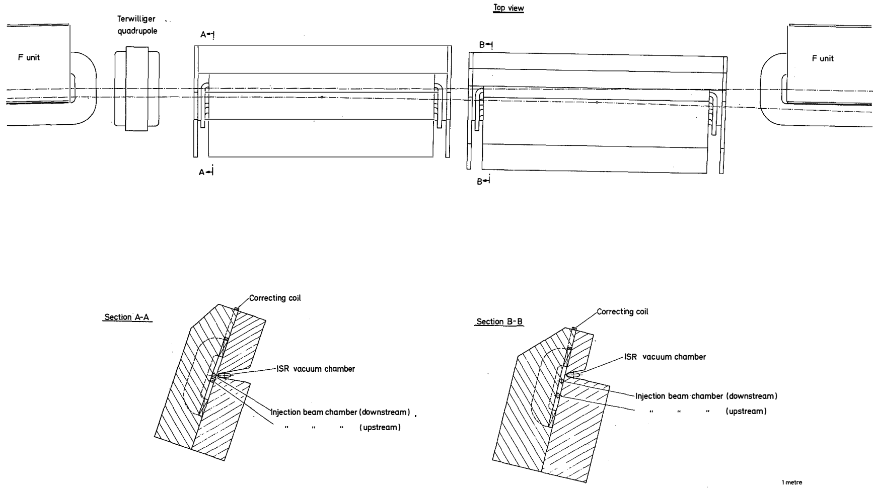
Fig. 3 View and cross-section of steel septum magnets
