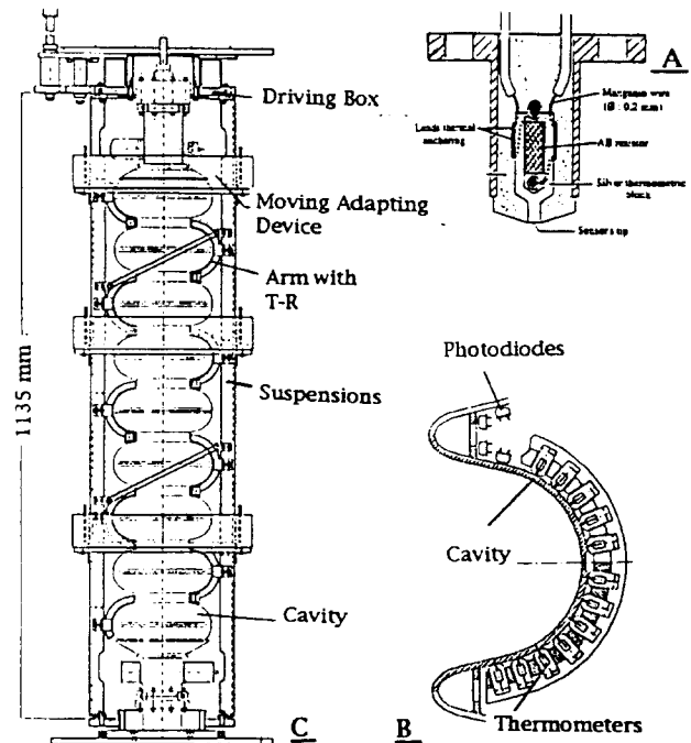
Figure 1: (A) A superfluid He scanning thermometer. (B) A rotating arm. (C) The DESY rotating T-R mapping without rotating measuring cables.
