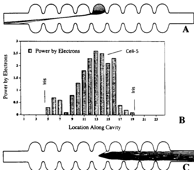
Figure 4: (A) FE electron trajectories of an emitter located at S_o=8 cm. (B) Power distribution contributed by impacting FE electrons from S_o=8 cm. (C) Electron trajectories, S_o=9 cm. for the heating shown in figure 3 is successfully identified.
