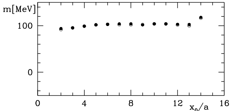
Fig. 2. Same as fig. 1, but using the O(a) improved action and the improved axial current \mathcal{A}_\mu^a/Z_A and density \mathcal{P}^a/Z_P with c_{sw} = 1.60 and c_A = -0.027 .
