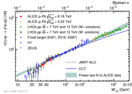
Figure 1. Energy dependence of exclusive J/\psi production in p–Pb ultra-peripheral collisions [1]. The data are described by a power-law growth in the range of Bjorken- x of 10^{-5} \lesssim x \lesssim 10^{-2} .
