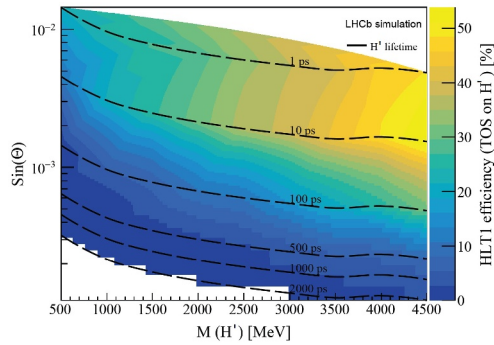
Figure 7. Proportion of events triggered by the HLT1 decision on the H' decay products (Trigger on Signal (TOS)) [3]
