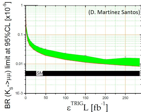
Figure 3. The sensitivity (illustrated by the green band) to the K_s^0 \rightarrow \mu^+ \mu^- branching fraction as function of the trigger efficiency \times luminosity. The black line demarcates the SM’s predictions [11].
