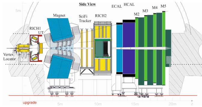
Figure 1. The LHCb detector operating during the Run 3 [6].
