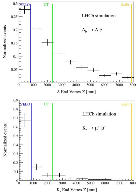
Figure 4. \Lambda^0 (top) and K_s^0 (bottom) reconstructible candidates charted against the decay vertex position. The candidates of \Lambda^0 disintegrate into a proton-pion pair, whereas the K_s^0 candidates devolve into two charge muons. The vertical colored demarcations denote the placements of the Velo, UT, and SciFi detectors on the Z-axis [3].
