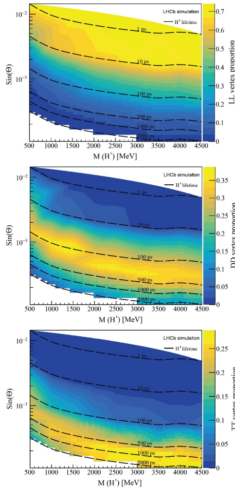
Figure 6. Reconstructibility of the decay vertex of the H' particle as a function of its mass and lifetime. Decay topologies are shown, from top to bottom, in the order: LL , DD , TT , corresponding to the track types of the two muons. [3]
