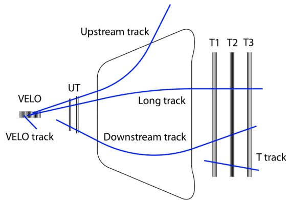
Figure 2. Definition of the track types in the LHCb detector, according to which detectors are hit. The different tracker layers and the magnet, in the centre, are sketched.
