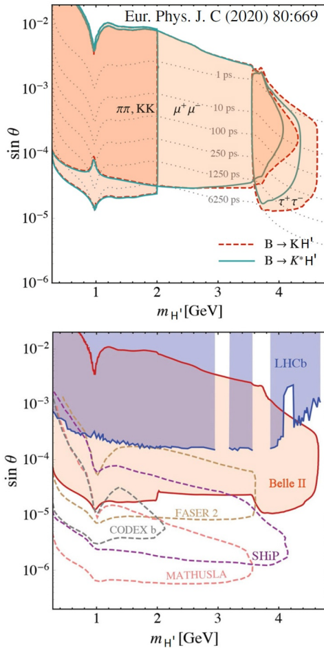
Figure 5. Parameter space regions for the B \rightarrow H'K and B \rightarrow H'K^* decay channels (top) and sensitivity to the H' displaced vertex by different present and future experiments (bottom), (Figs. adapted from [8]).
