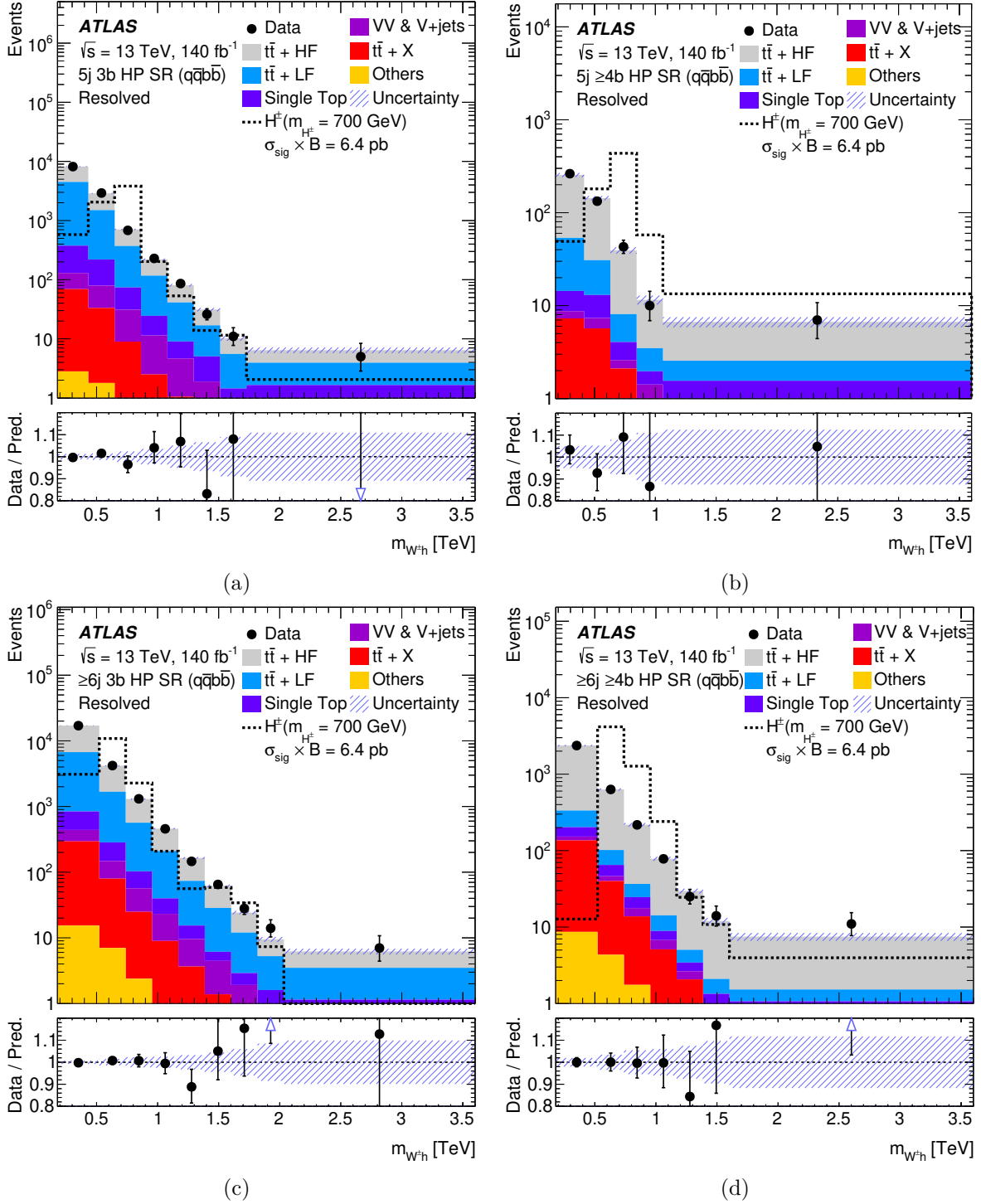
Figure 10. The m_{W^\pm h} distributions in the high-purity signal regions (HP SR) of the resolved q\bar{q}b\bar{b} event categories. The term ‘Others’ summarises events from tHj b , tWh , t\bar{t}\bar{t} , and SM Vh production. The background prediction is shown after a background-only maximum-likelihood fit to data. The lower panels show the ratio of the observed to the estimated SM background. The shaded bands show the total post-fit uncertainty in the background. The expected signal contribution assuming m_{H^\pm} = 700 GeV, normalised to a cross-section times branching ratio ( \sigma_{\text{sig}} \times B ) of 6.4 pb, is shown as a dashed histogram.
