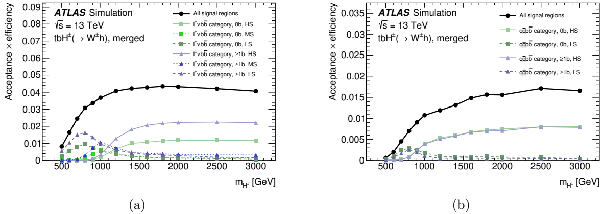
Figure 6. Product of acceptance and efficiency for pp \rightarrow tbH^\pm(\rightarrow W^\pm h) as a function of the charged Higgs boson mass for (a) the merged l^\pm\nu b\bar{b} high-NN score (HS), medium-NN score (MS) and low-NN score (LS) signal regions, and (b) the merged q\bar{q}b\bar{b} high-NN score and low-NN score signal regions.
