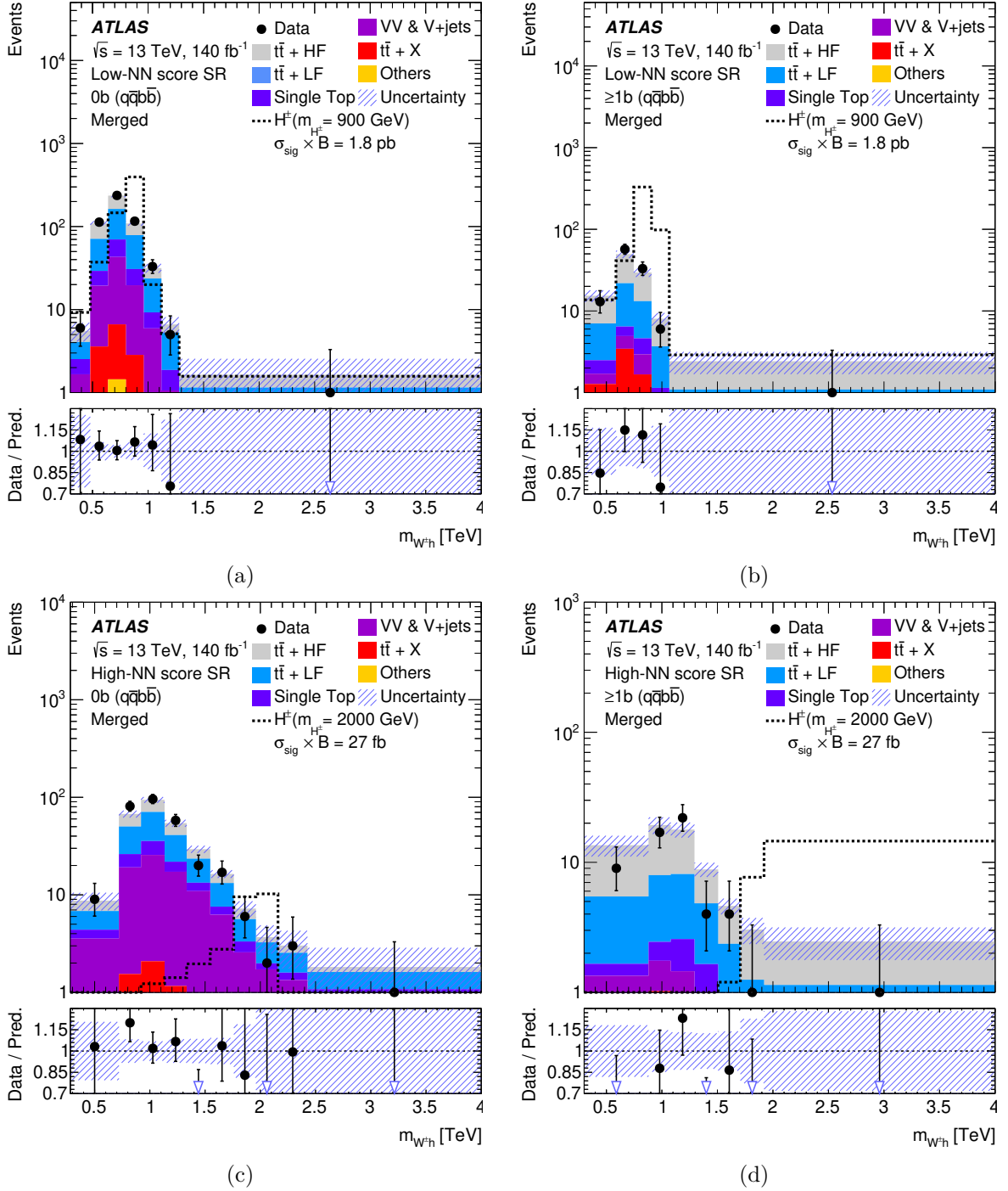
Figure 12. The m_{W^{\pm}h} distributions in the low-NN-score signal regions (low-NN-score SRs) and high-NN-score signal regions (high-NN-score SRs) of the merged q\bar{q}b\bar{b} event categories. The term ‘Others’ summarises events from tHj\bar{b} , tWh , t\bar{t}\bar{t} , and SM Vh production. The background prediction is shown after a background-only maximum-likelihood fit to data. The lower panels show the ratio of the observed to the estimated SM background. The shaded bands show the total post-fit uncertainty in the background. The expected signal contributions assuming m_{H^{\pm}} = 900 GeV and m_{H^{\pm}} = 2000 GeV, normalised to cross-section times branching ratio ( \sigma_{\text{sig}} \times B ) values of 1.8 pb and 27 fb respectively, are shown as dashed histograms.
