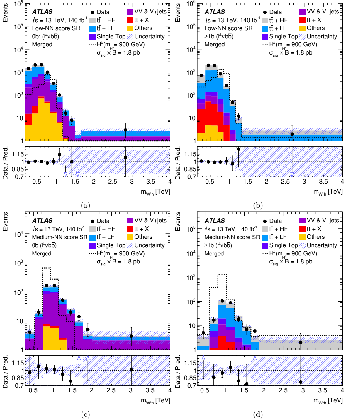
Figure 13. The m_{W^{\pm h}} distributions in the low-NN-score signal regions (low-NN-score SRs) and medium-NN-score signal regions (medium-NN-score SRs) of the merged \ell^{\pm} \nu b \bar{b} event categories. The term ‘Others’ summarises events from tHj b , tWh , t\bar{t}t\bar{t} , and SM Vh production. The background prediction is shown after a background-only maximum-likelihood fit to data. The lower panels show the ratio of the observed to the estimated SM background. The shaded bands show the total post-fit uncertainty in the background. The expected signal contribution assuming m_{H^{\pm}} = 900 \text{ GeV} , normalised to a cross-section times branching ratio ( \sigma_{\text{sig}} \times B ) values of 1.8 pb, is shown as a dashed histogram.
