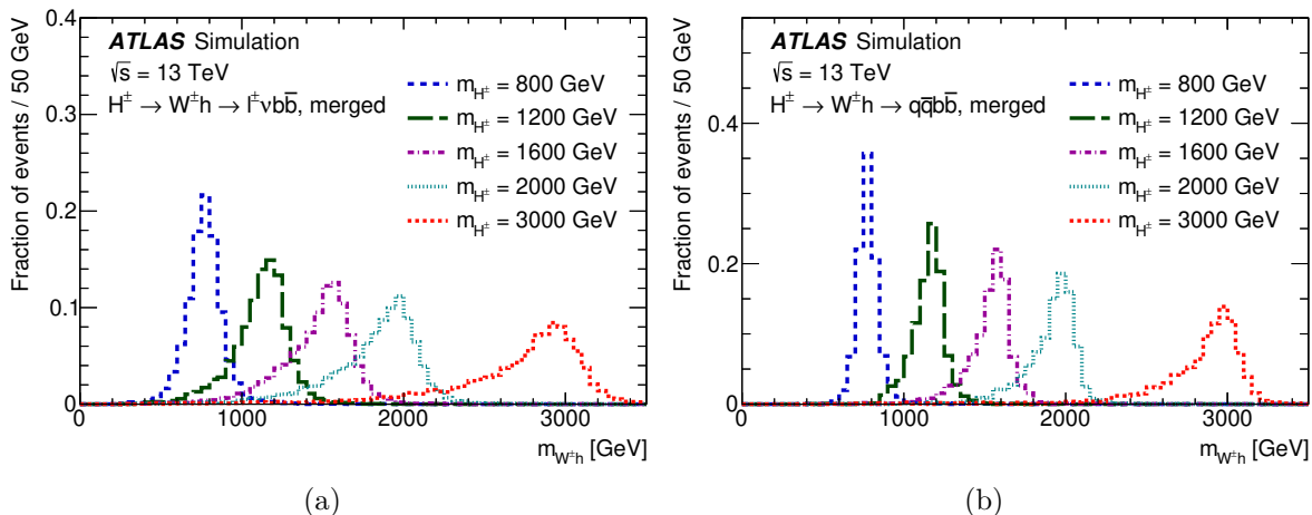
Figure 4. Distributions of the invariant mass of the (a) H^\pm \rightarrow W^\pm h \rightarrow \ell^\pm \nu b \bar{b} and (b) H^\pm \rightarrow W^\pm h \rightarrow q \bar{q} b \bar{b} signal hypotheses presented for a selection of different charged Higgs boson pole masses. The final states are reconstructed using either a charged lepton, a neutrino candidate, and one large- R jet (for the \ell^\pm \nu b \bar{b} channel) or via two large- R jets (for the q \bar{q} b \bar{b} channel) for events entering the merged analysis regions. All distributions are normalised to unit area.
