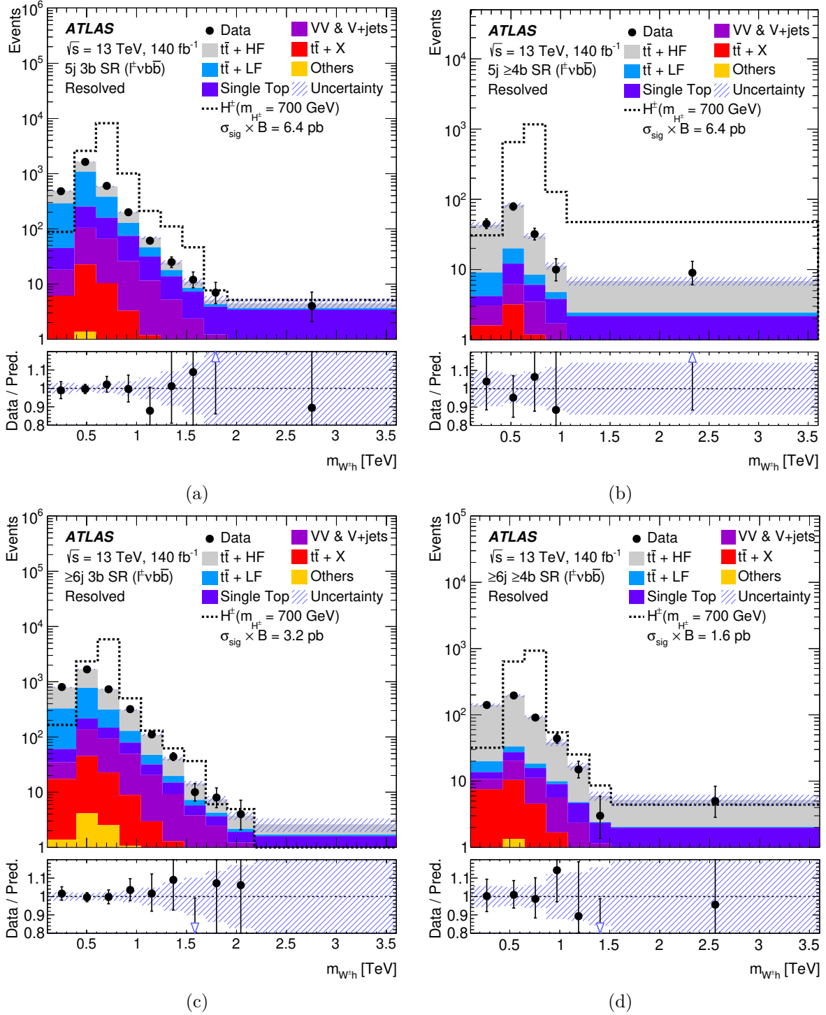
Figure 11. The m_{W^{\pm}h} distributions in the signal regions (SRs) of the resolved l^{\pm}\nu b\bar{b} event categories. The term ‘Others’ summarises events from tHj b , tWh , t\bar{t}t , and SM Vh production. The background prediction is shown after a background-only maximum-likelihood fit to data. The lower panels show the ratio of the observed to the estimated SM background. The shaded bands show the total post-fit uncertainty in the background. The expected signal contribution assuming m_{H^{\pm}} = 700 GeV, normalised to different values of the cross-section times branching ratio ( \sigma_{\text{sig}} \times B ), is shown as a dashed histogram.
