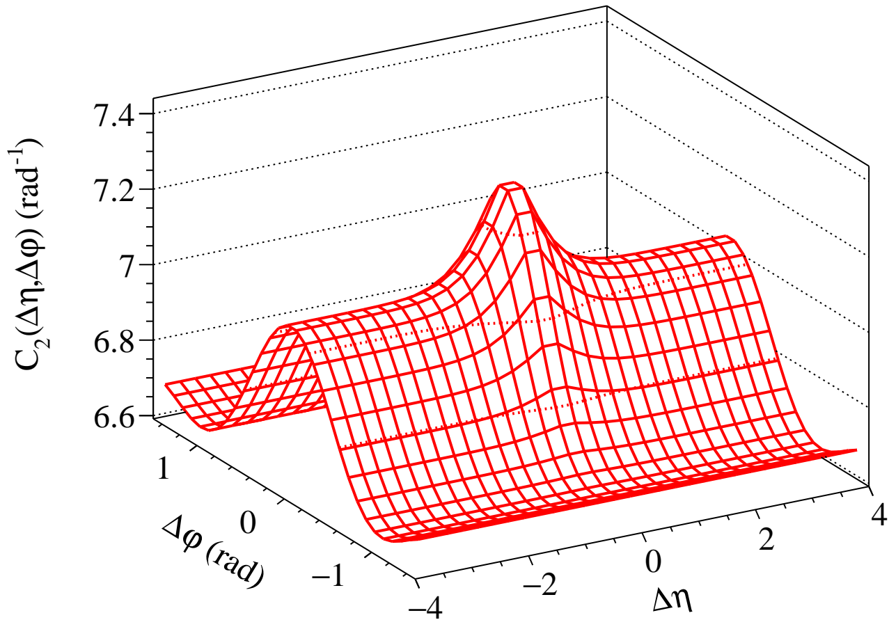
Fit function:: Flow Bkg + Nearside peak
